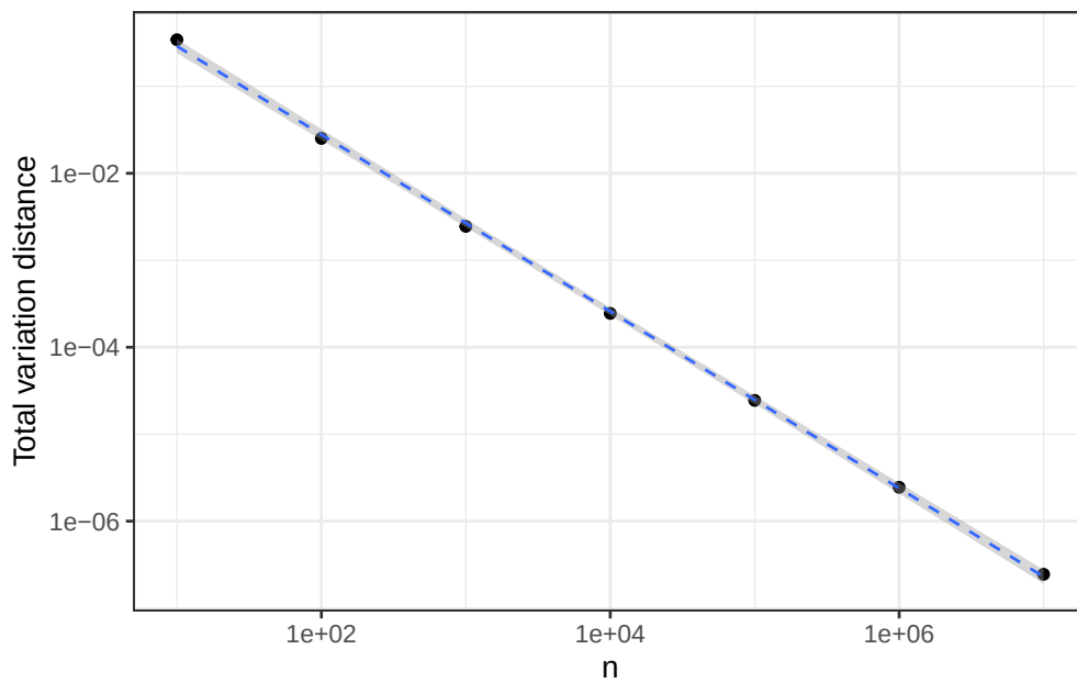
FIGURE I.3 : Law of rare events : distance between Binomial( n, 5/n ) and Poisson(5) as a function of n
