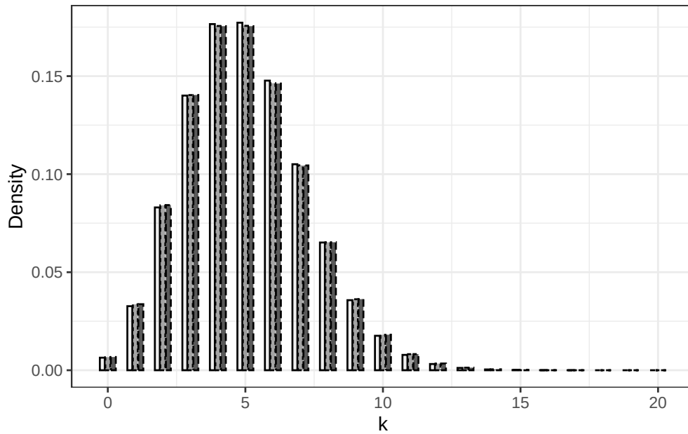
FIGURE I.2 : Probability mass functions of Binomial(250,0.02) (left), Binomial(2500,0.002) (middle) and Poisson(5) (right)
