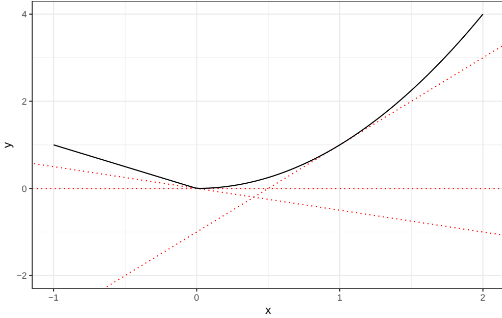
FIGURE 4.1 : The function f : x \mapsto \mathbb{1}_{x < 0}|x| + \mathbb{1}_{x \geq 0}x^2 is convex, continuous. It is differentiable everywhere except at x = 0 . The dotted lines define affine functions that are below the curve y = f(x) . The dotted lines define supporting hyperplanes for the epigraph of f .
