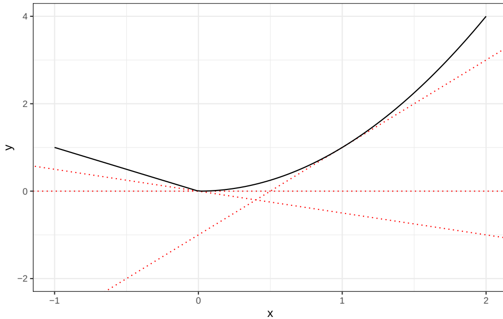
Figure 4.1: The function f : x \mapsto \inf_{x < 0} |x| + \inf_{x \geq 0} x^2 is convex, continuous. It is differentiable everywhere except at x = 0 . The dotted lines define affine functions that are below the curve y = f(x) . The dotted lines define supporting hyperplanes for the epigraph of f .
