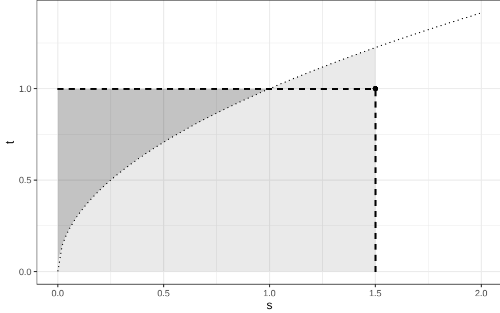
Figure 4.2: Graphical illustration of Young's inequality. We choose p = \lceil rp \rceil and q = \lceil rq \rceil , x = \lceil rx \rceil and y = \lceil ry \rceil . The black point is located at (x, y)^T . The product xy equals the area of the rectangle located between the origin and (x, y)^T (delimited by the dashed segments). The dotted line represents function s \mapsto s^{p-1} , and interchanging the axes, the function t \mapsto t^{q-1} = t^{1/(p-1)} . The area of the light grey surface under the dotted line equals \frac{x^p}{p} = \int_0^x s^{p-1} ds , while the area of the darker grey surface below line y = 1 and above the dotted line, equals \frac{y^q}{q} = \int_0^y t^{q-1} dt . The union of the two disjoint surfaces covers the rectangle located between the origin and (x, y)^T . Equality occurs when the dotted line passes through (x, y)^T , that is when y = x^{p-1} .
