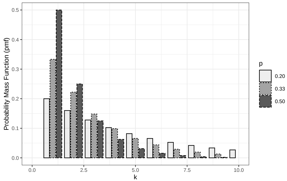
FIGURE 5.3 : Geometric probability mass functions with different values of parameter p : 1/2, 1/3, 1/5 . The probability mass function equals p \times (1 - p)^{k-1} at k \geq 1 . The mode is achieved at k = 1 whatever the value of p . The expectation equals 1/p
