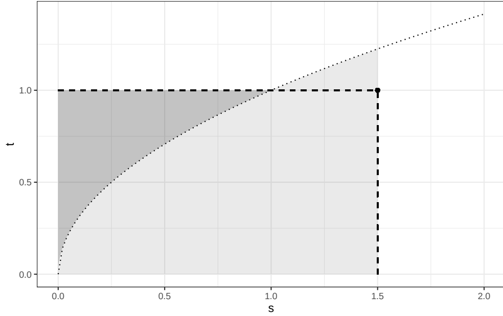
FIGURE 4.2 : Graphical illustration of Young's inequality. We choose p = \frac{r}{r-1} and q = \frac{r}{r-1} , x = \frac{r}{r-1} s and y = \frac{r}{r-1} t . The black point is located at (x, y)^T . The product xy equals the area of the rectangle located between the origin and (x, y)^T (delimited by the dashed segments). The dotted line represents function s \mapsto s^{p-1} , and interchanging the axes, the function t \mapsto t^{q-1} = t^{1/(p-1)} . The area of the light grey surface under the dotted line equals \frac{x^p}{p} = \int_0^x s^{p-1} ds , while the area of the darker grey surface below line y = 1 and above the dotted line, equals \frac{y^q}{q} = \int_0^y t^{q-1} dt . The union of the two disjoint surfaces covers the rectangle located between the origin and (x, y)^T . Equality occurs when the dotted line passes through (x, y)^T , that is when y = x^{p-1} .
