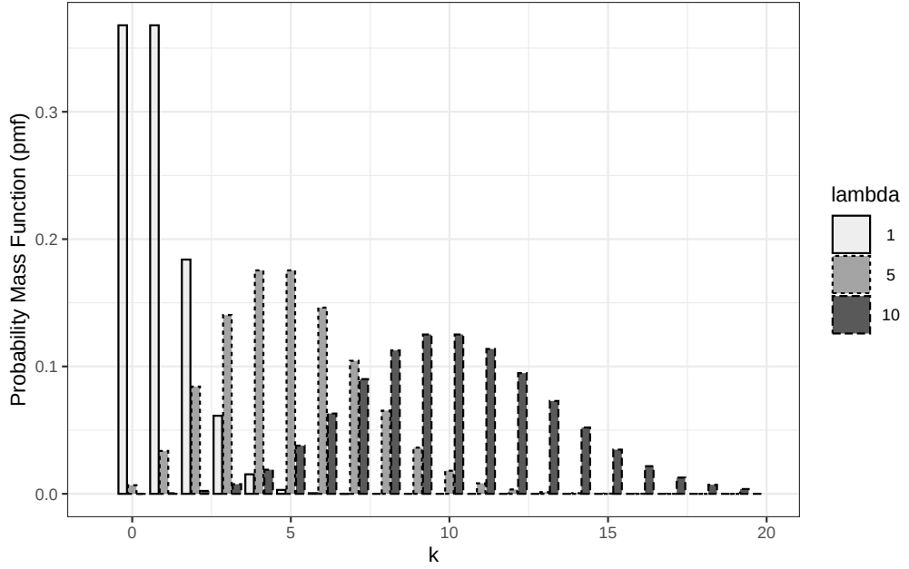
FIGURE 5.2 : Poisson probability mass functions with different values of parameter : 1, 5, 10. Recall that the parameter of a Poisson distribution equals its expectation and its variance. The probability mass function of a Poisson distribution achieves its maximum (called the mode) close to its expectation.
