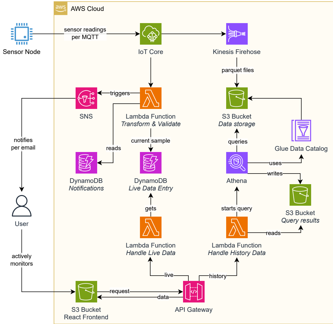
Figure 1. Cloud processing architecture depicting the sensor node, backend services, and user interaction components.
