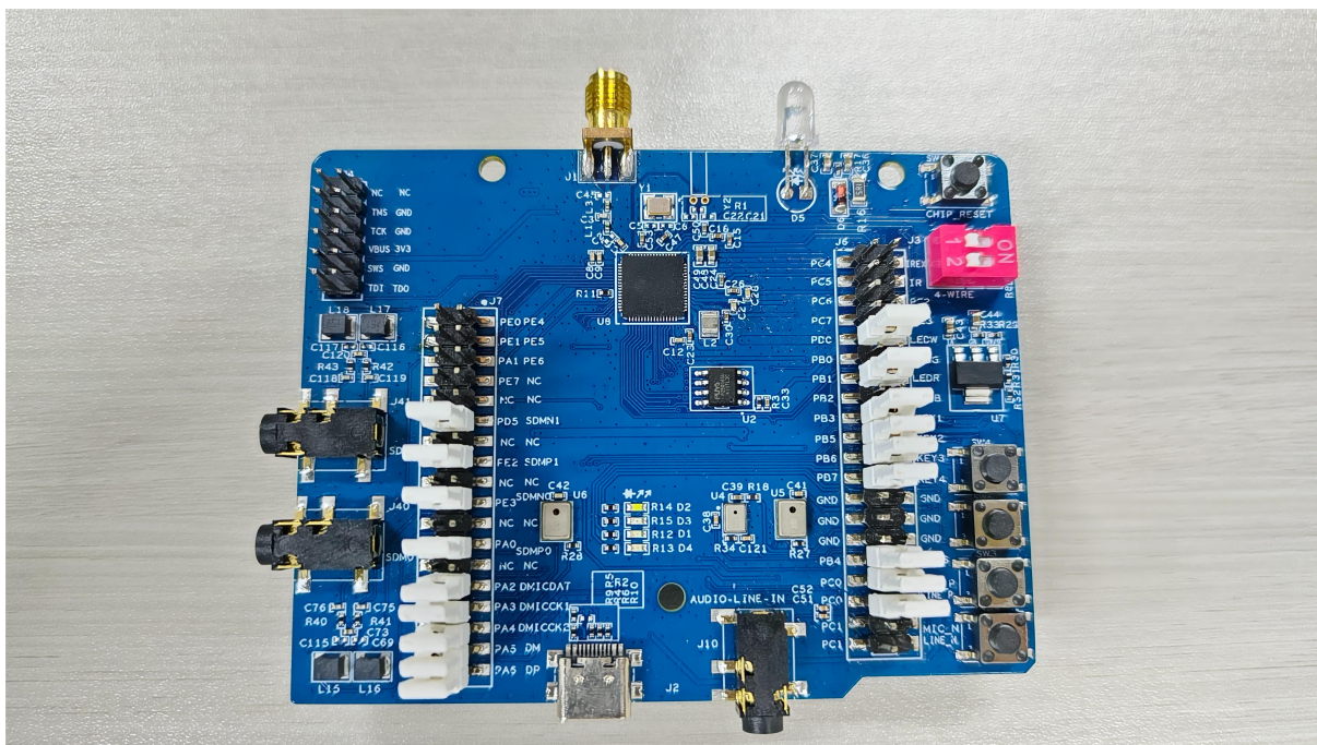
Figure 6: TL321x-Development-Board-Front
