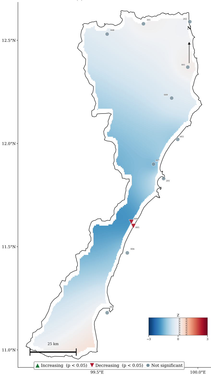
(a) Standard MK — Z Statistic
