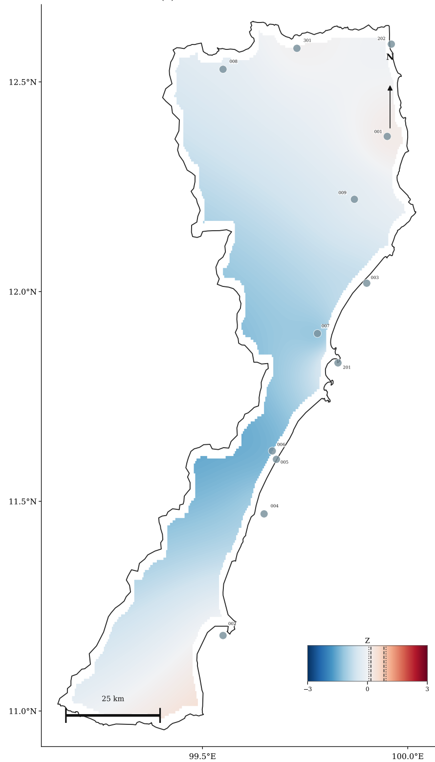
(b) Modified MK — Z Statistic
