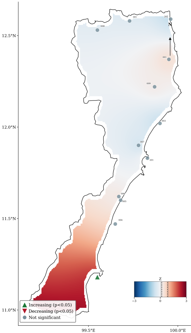
(a) Standard MK — Z Statistic
