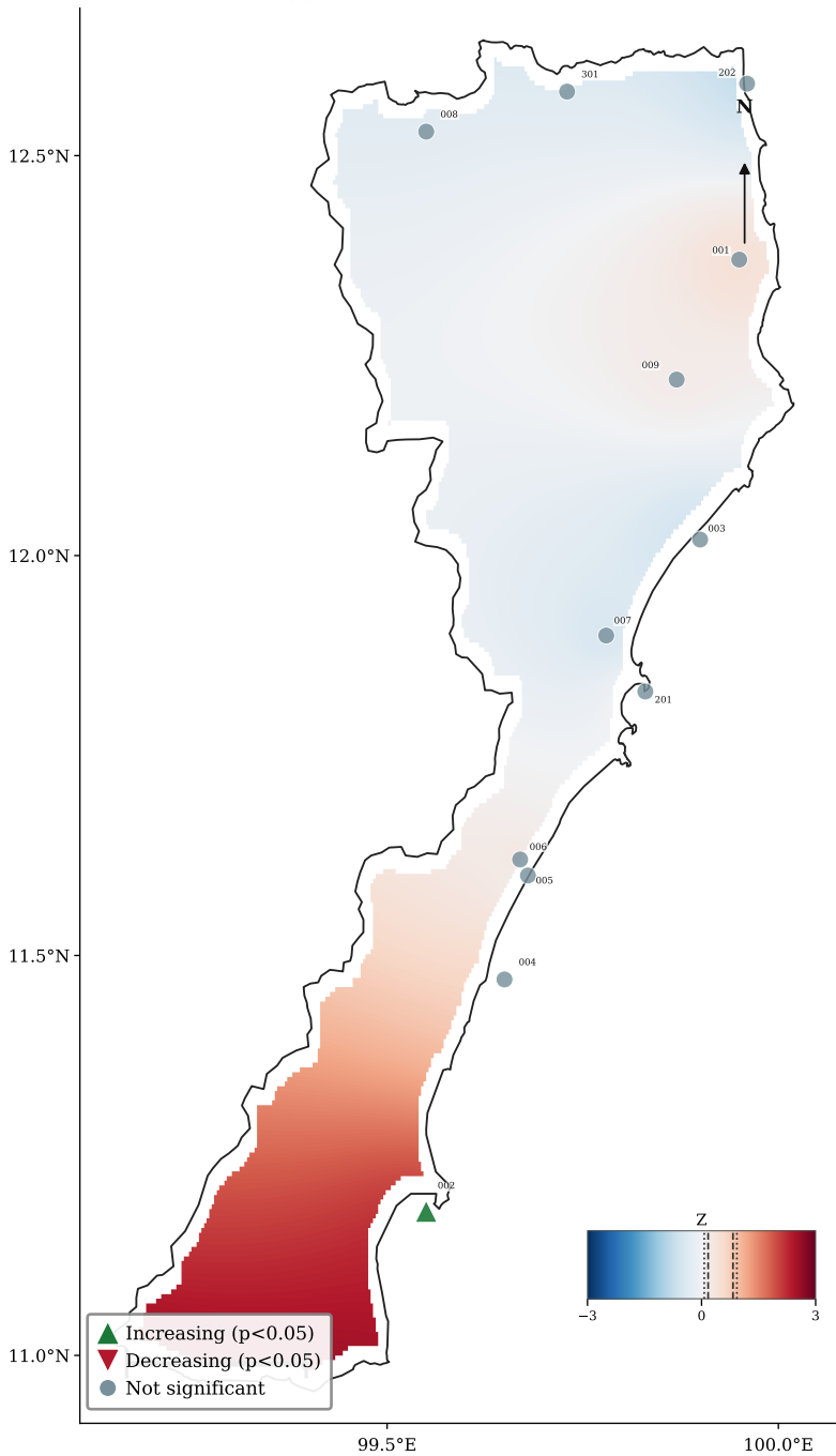
(b) Modified MK — Z Statistic
