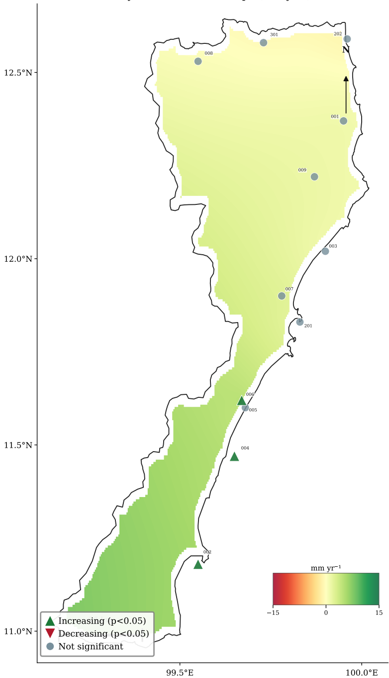
Dry Season — Sen's Slope ( \text{mm yr}^{-1} )
