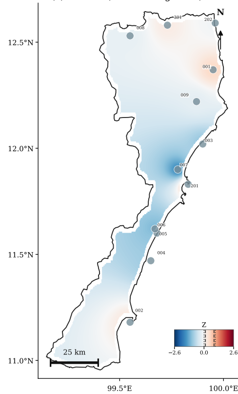
(c) PW-MK (Yue & Wang 2004) — Z
