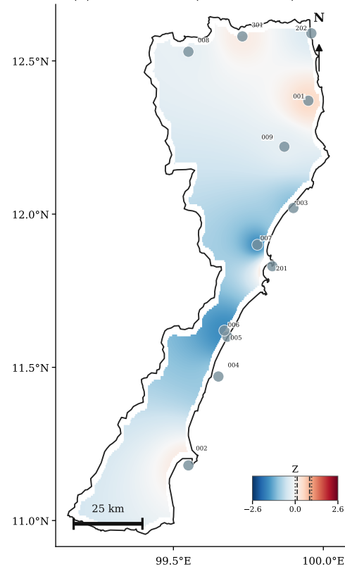
(b) Modified MK (Hamed 1998) — Z
