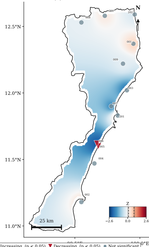
(a) Standard MK — Z
