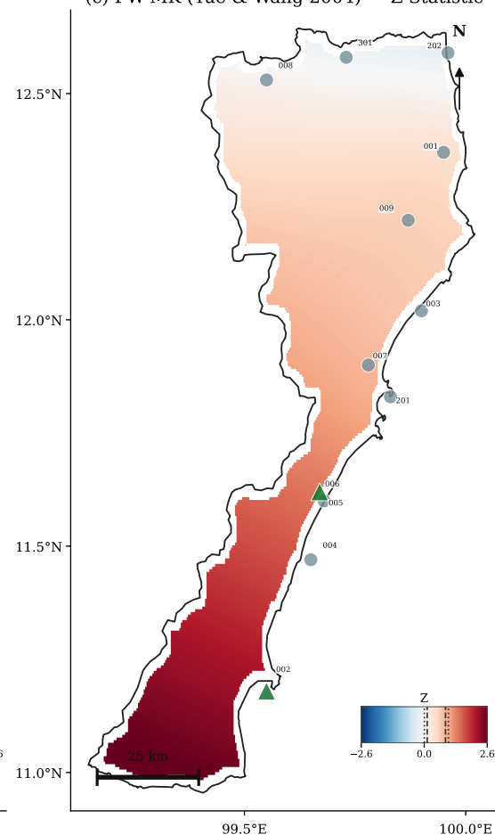
(c) PW-MK (Yue & Wang 2004) — Z Statistic
