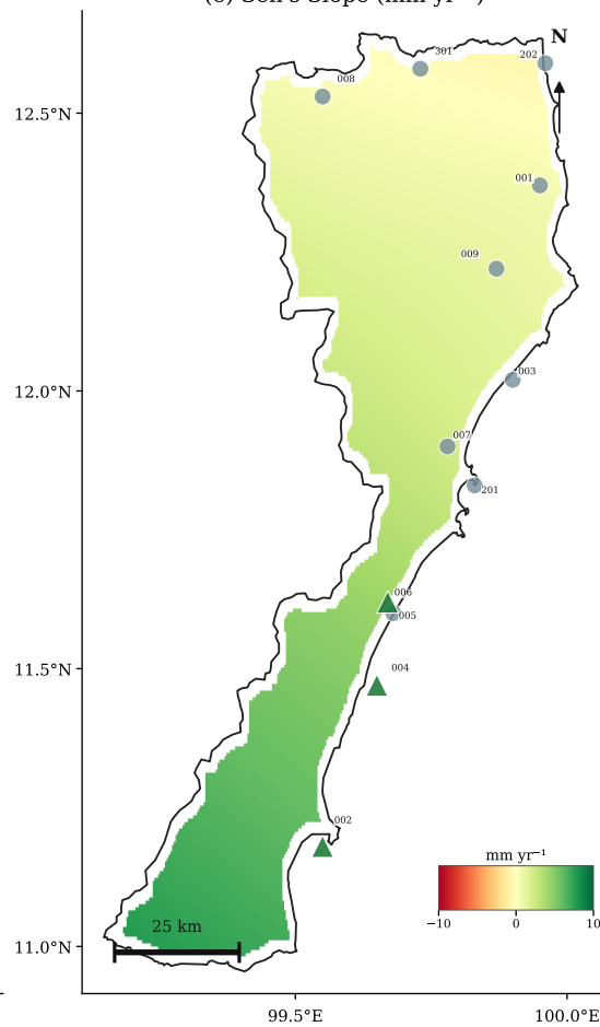
(e) Sen's Slope ( \text{mm yr}^{-1} )
