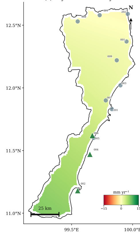
(c) Dry Season — mm yr -1
