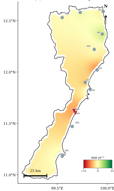
(b) Wet Season — mm yr -1
