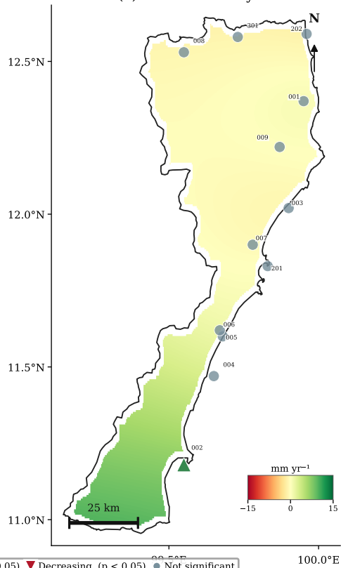
(a) Annual — mm yr -1
