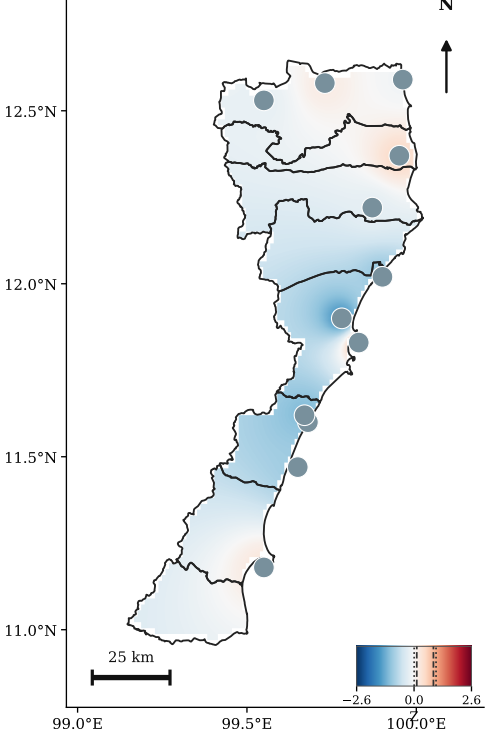
(c) PW-MK (Yue & Wang 2004) — Z Statistic
