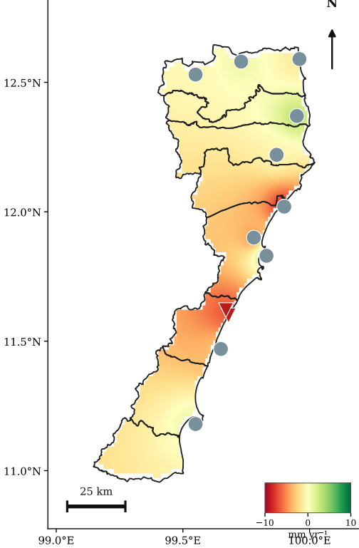
(e) Sen's Slope (mm yr -1 )
