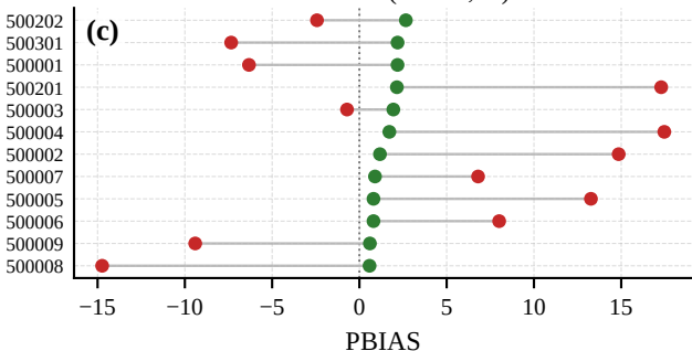
Percent Bias (PBIAS, %)
