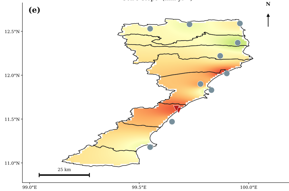
Sen's Slope ( \text{mm yr}^{-1} )
