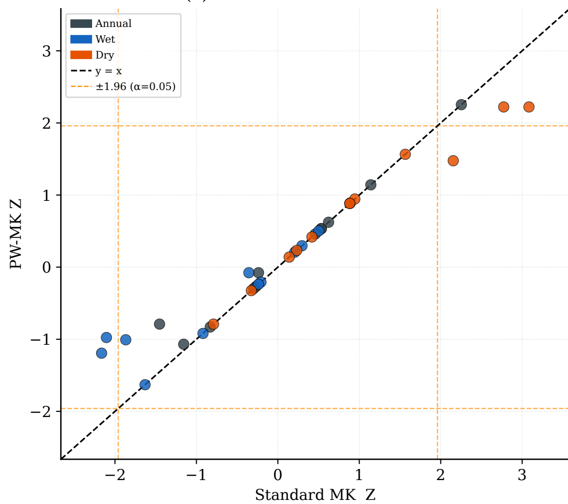
(b) PW-MK Z vs Standard MK Z
