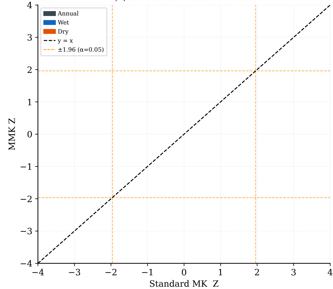
(a) MMK Z vs Standard MK Z
