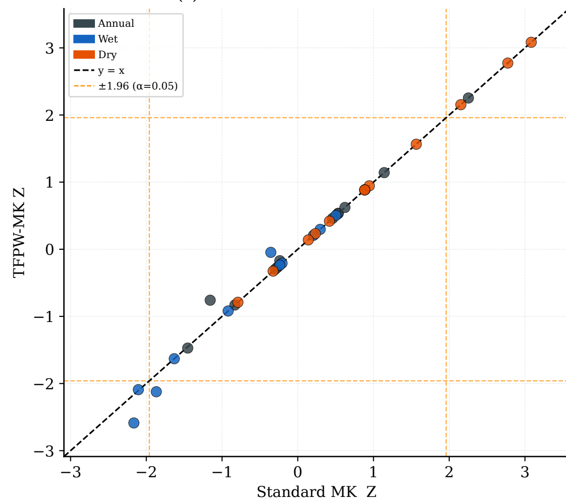
(c) TFPW-MK Z vs Standard MK Z
