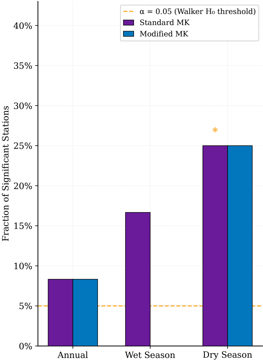
(a) Field Significance — Fraction Significant
