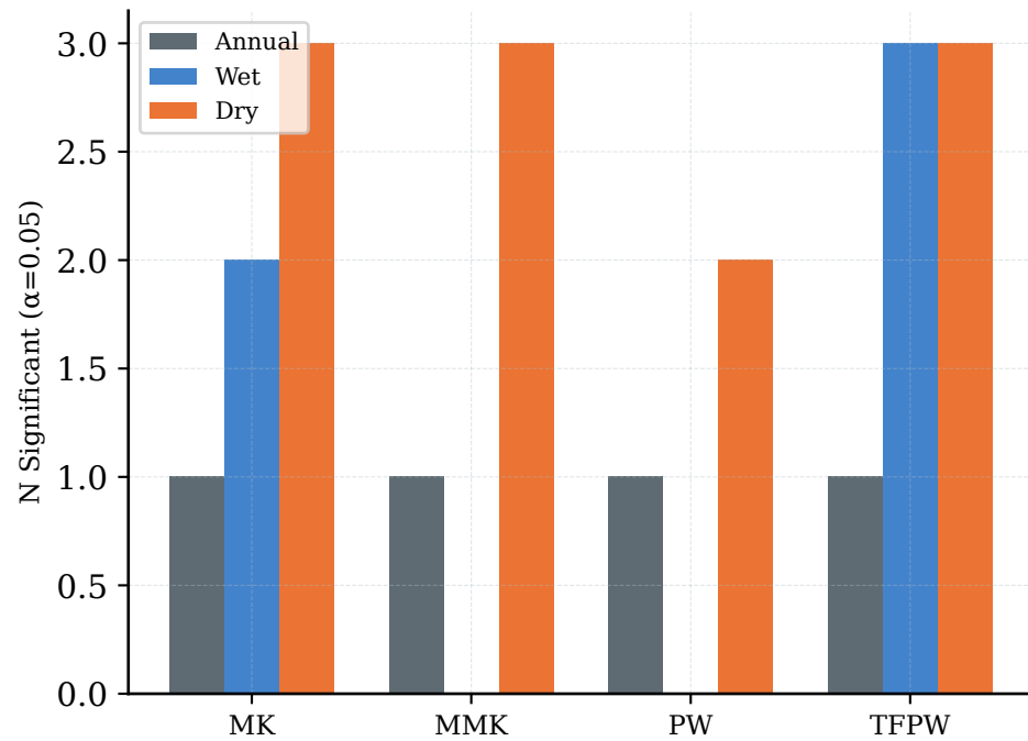
(a) N Significant by Method
