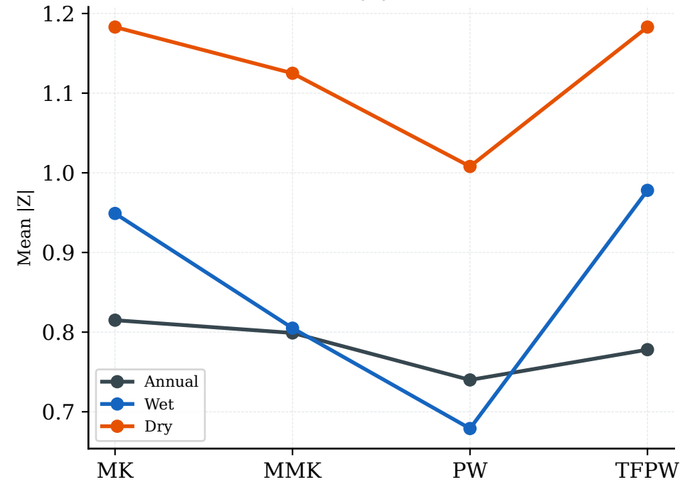
(b) Mean |Z| by Method
