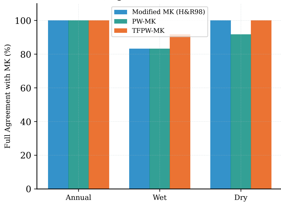
(c) Agreement Rate with MK
