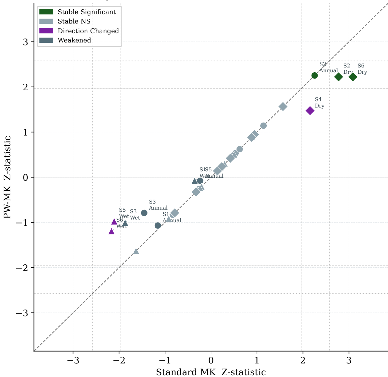
Figure 3: Standard MK vs PW-MK — Z-statistic
