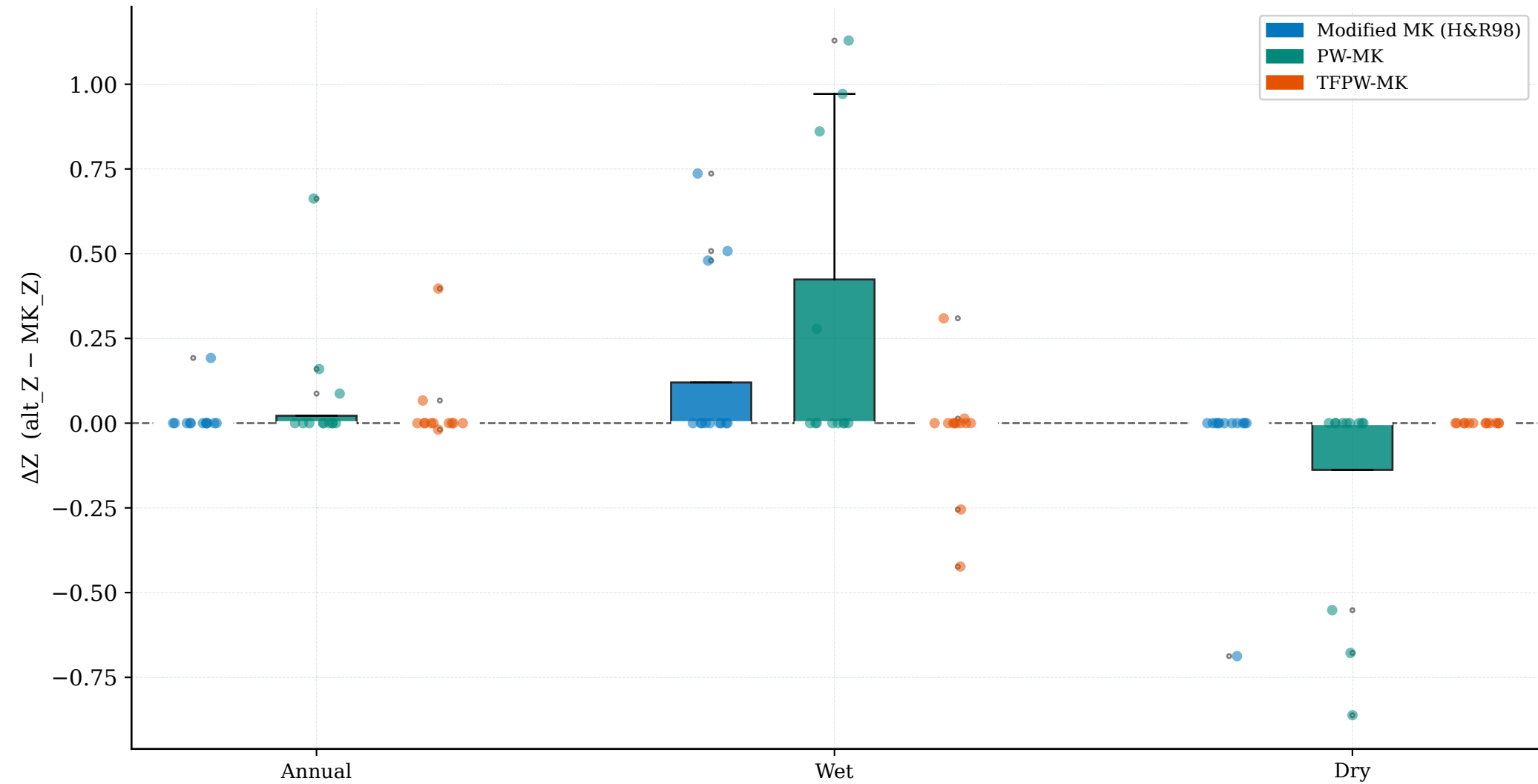
Figure 5: \Delta Z Distribution — Method Correction Effect on Z-statistic
