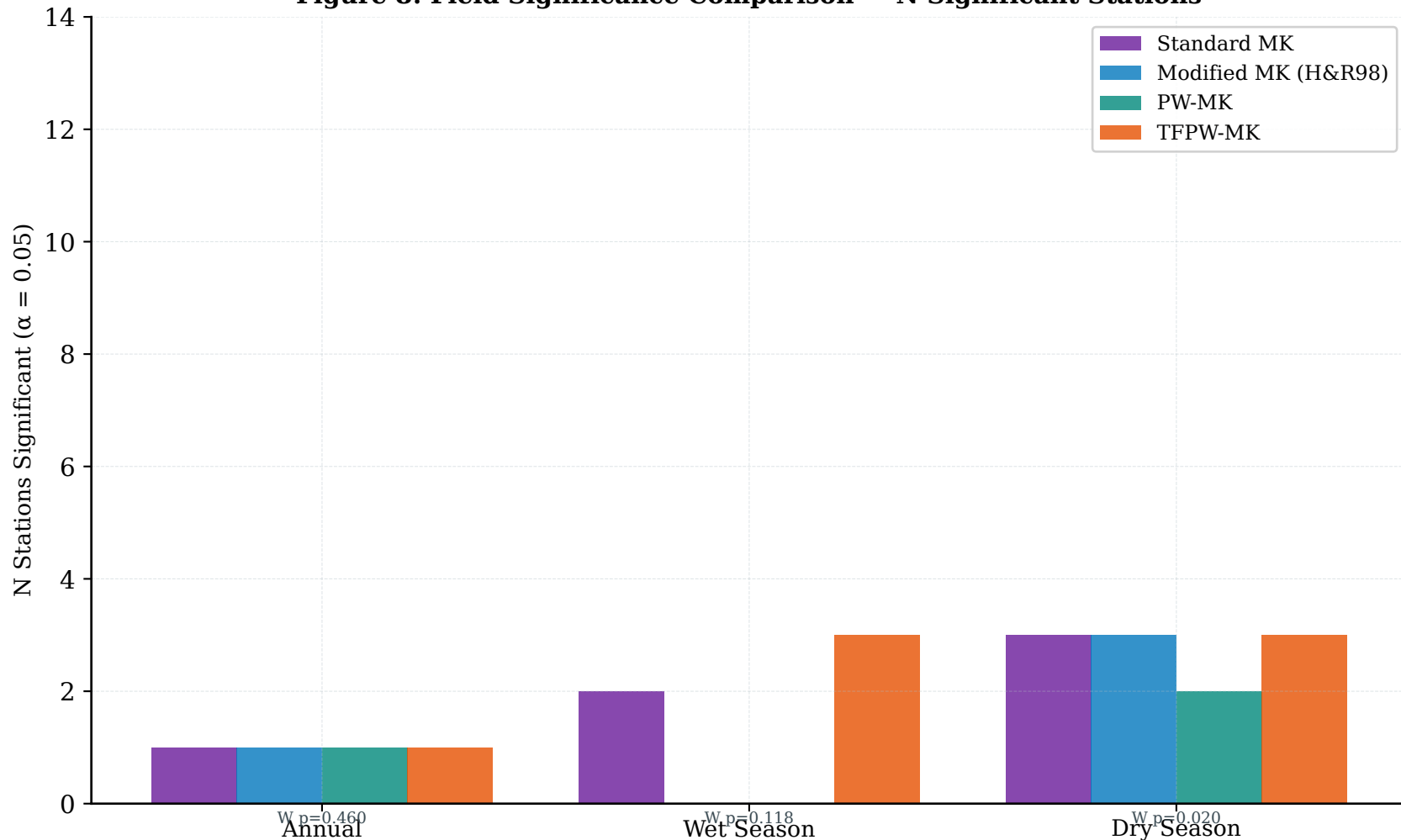
Figure 8: Field Significance Comparison — N Significant Stations
