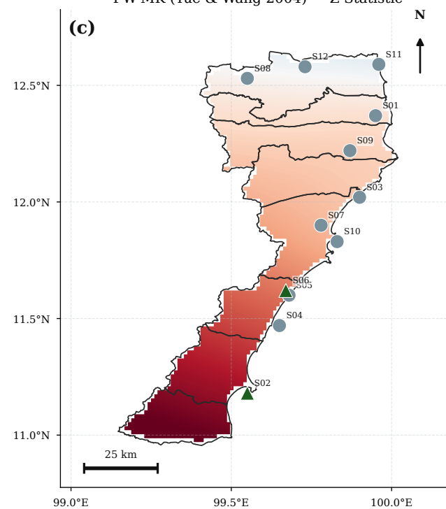
PW-MK (Yue & Wang 2004) — Z Statistic
