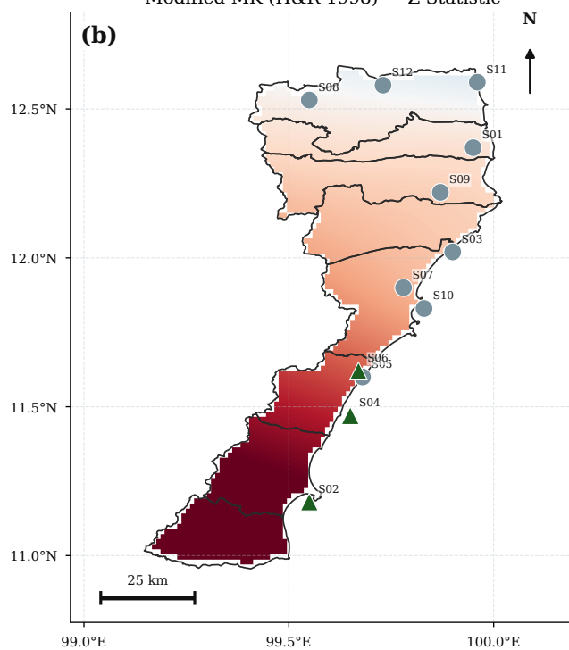
Modified MK (H&R 1998) — Z Statistic
