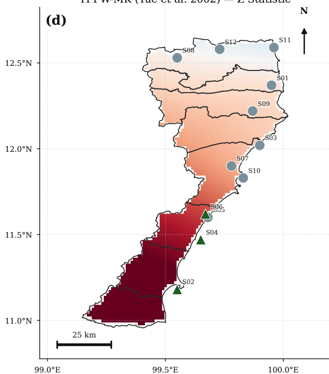
TFPW-MK (Yue et al. 2002) — Z Statistic
