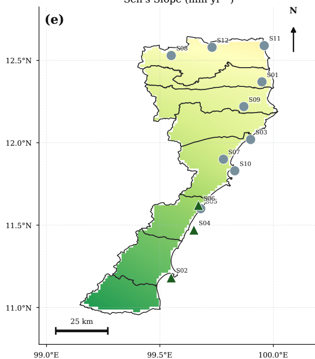
Sen's Slope (mm yr -1 )
