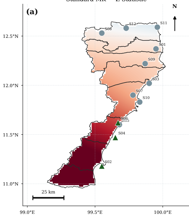
Standard MK — Z Statistic
