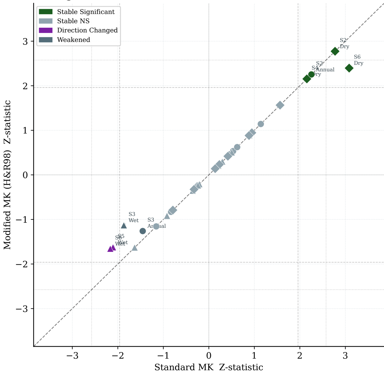
Figure 2: Standard MK vs Modified MK (H&R98) — Z-statistic
