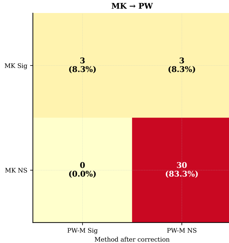
Figure 9: Significance Transition Matrix (MK → Alternative Method)
