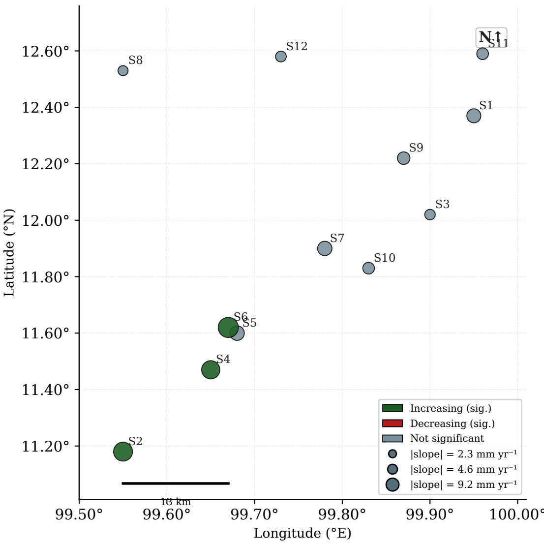
(c) Dry Season — Sen's Slope (MMK) 1981-2014
