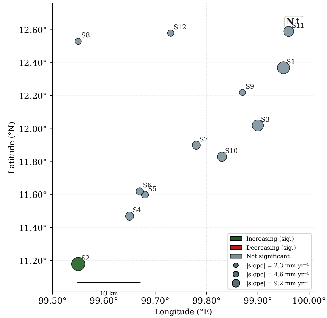
(a) Annual — Sen's Slope (MMK) 1981-2014
