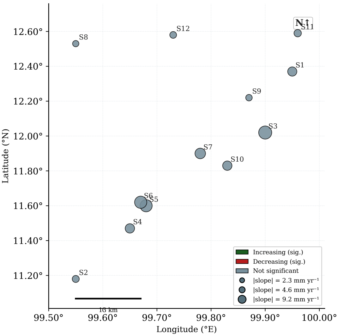
(b) Wet Season — Sen's Slope (MMK) 1981-2014
