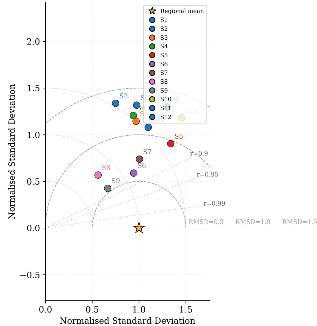
(a) Taylor Diagram — Annual (Jan-Dec) 1981-2014
