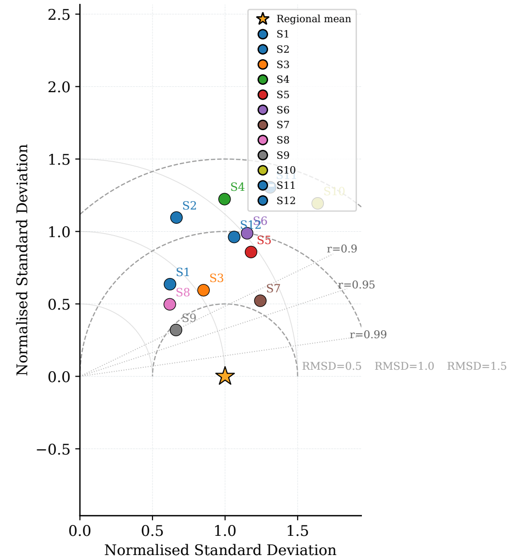
(c) Taylor Diagram — Dry Season (Nov-Apr) 1981-2014
