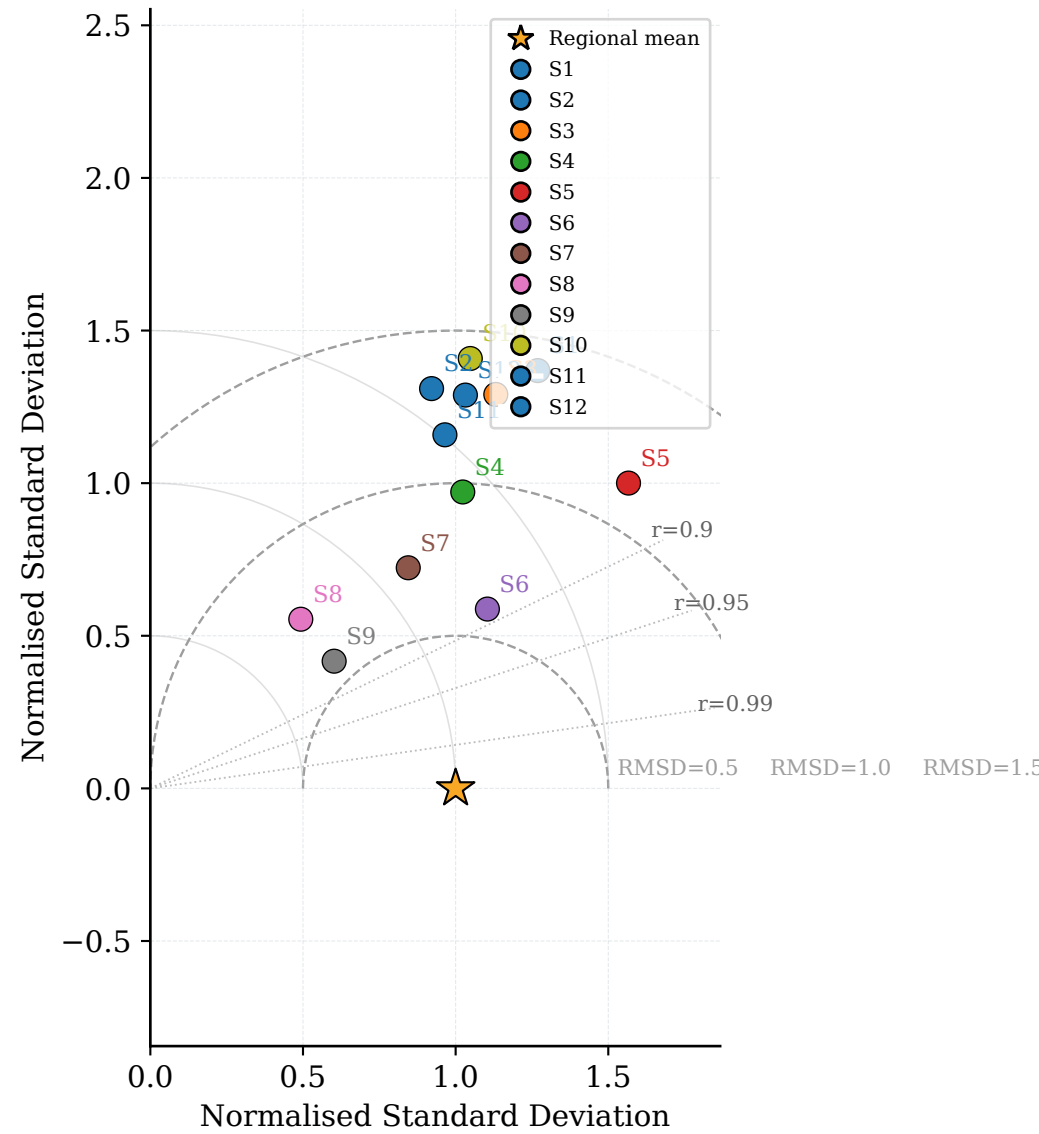
(b) Taylor Diagram — Wet Season (May-Oct) 1981-2014
