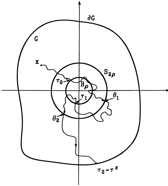
Figure 5.7.2: Stopping times \theta_m, \tau_m .
