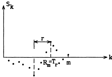
Figure 3.2.1: Maximal length segments.
