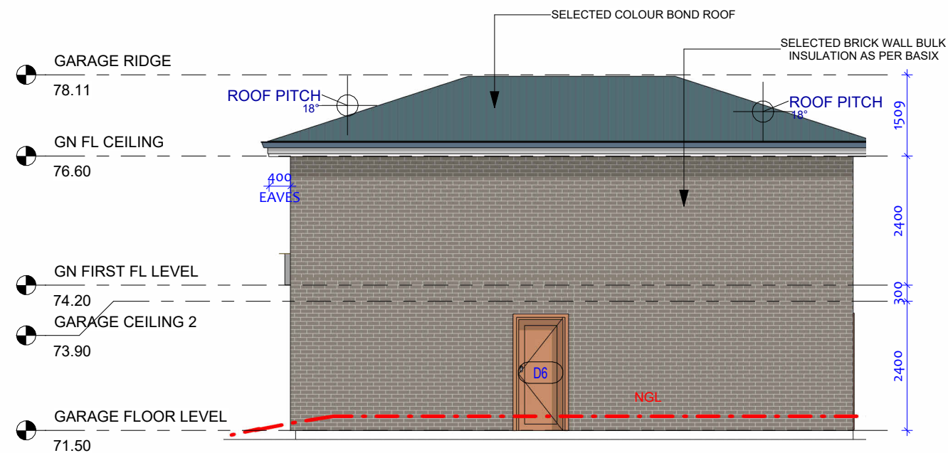
NORTH-WEST ELEVATION GRANNY
