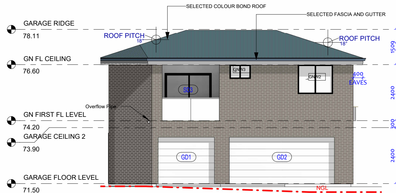
SOUTH-WEST ELEVATION GRANNY
