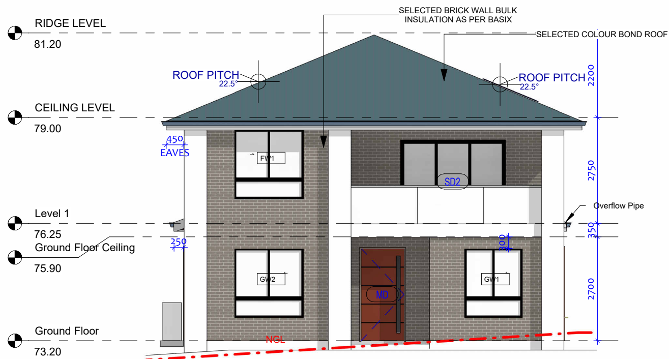
NORTH-EAST ELEVATION
