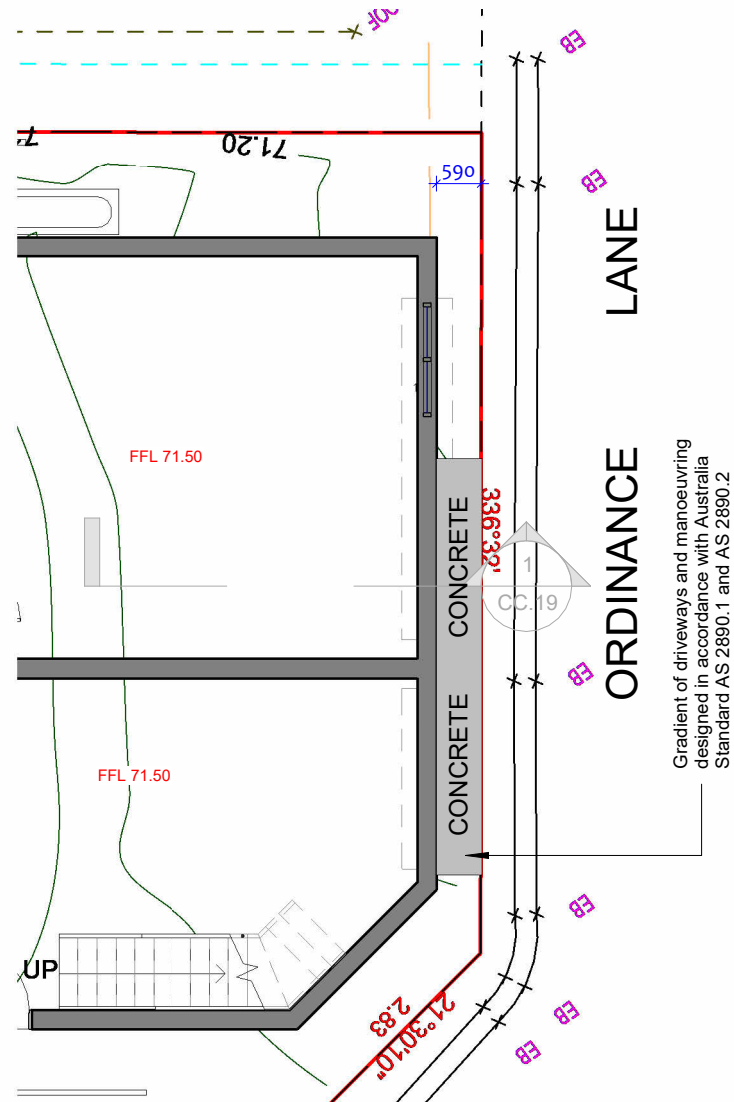
3 CC - DRIVEWAY PLAN 1 : 100
