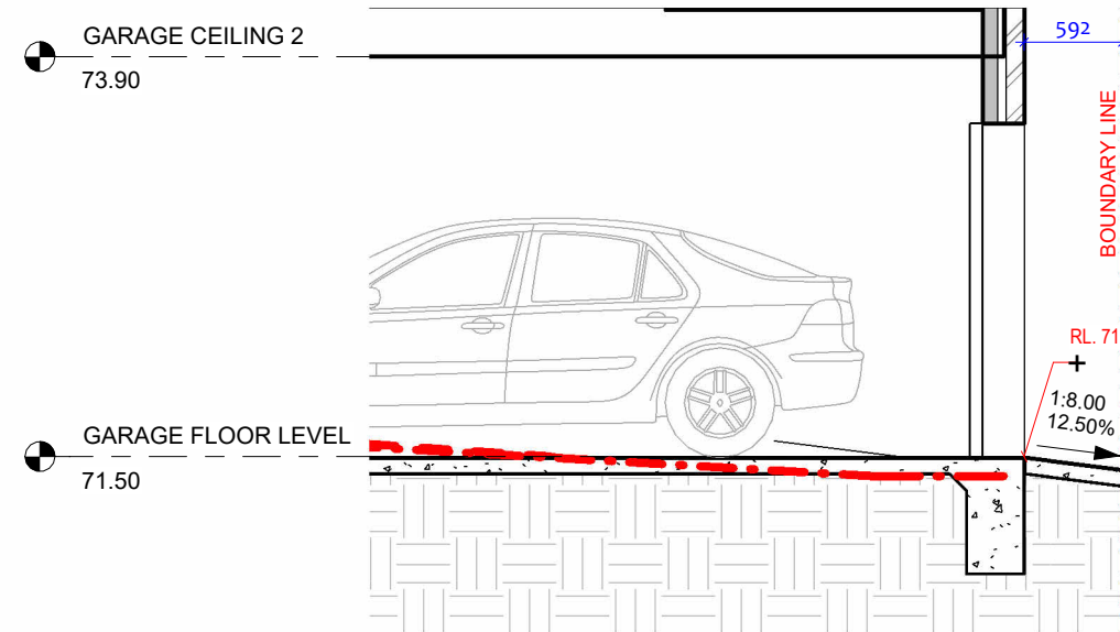
1 DRIVEWAY SECTION 1 : 50
