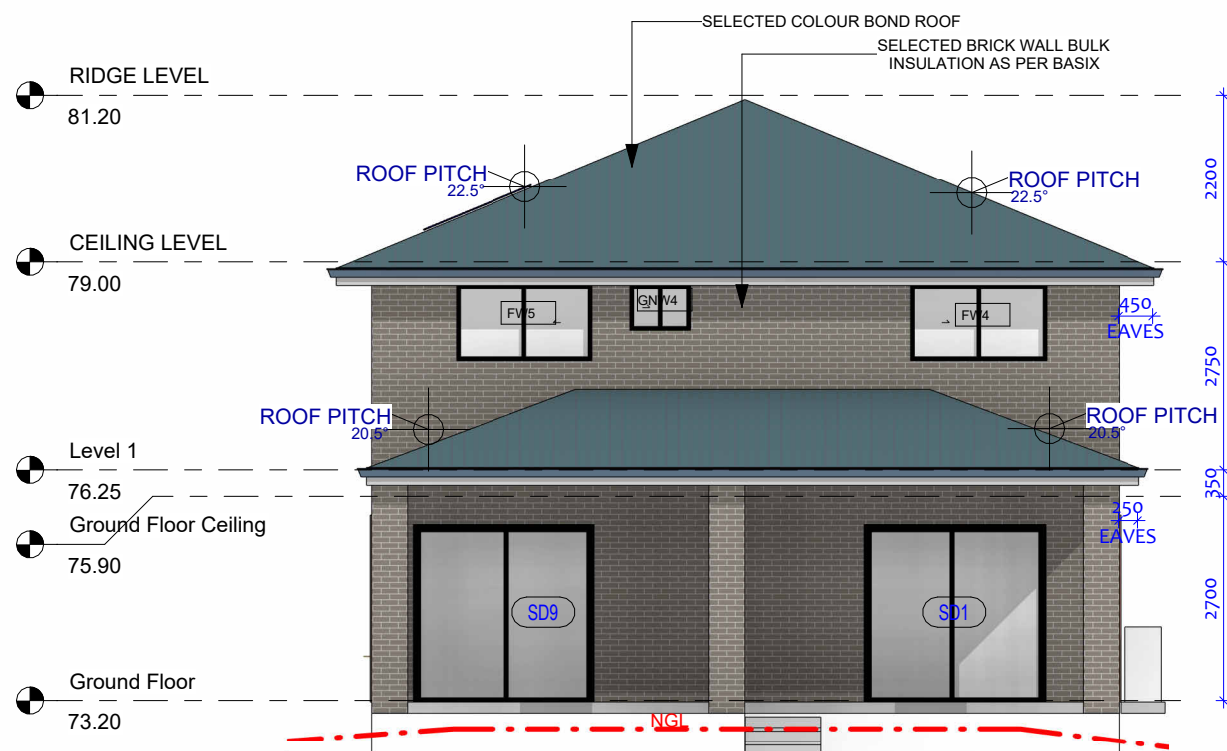
SOUTH-WEST ELEVATION
