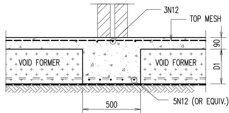
INTERNAL BEAM – 'IB4'
