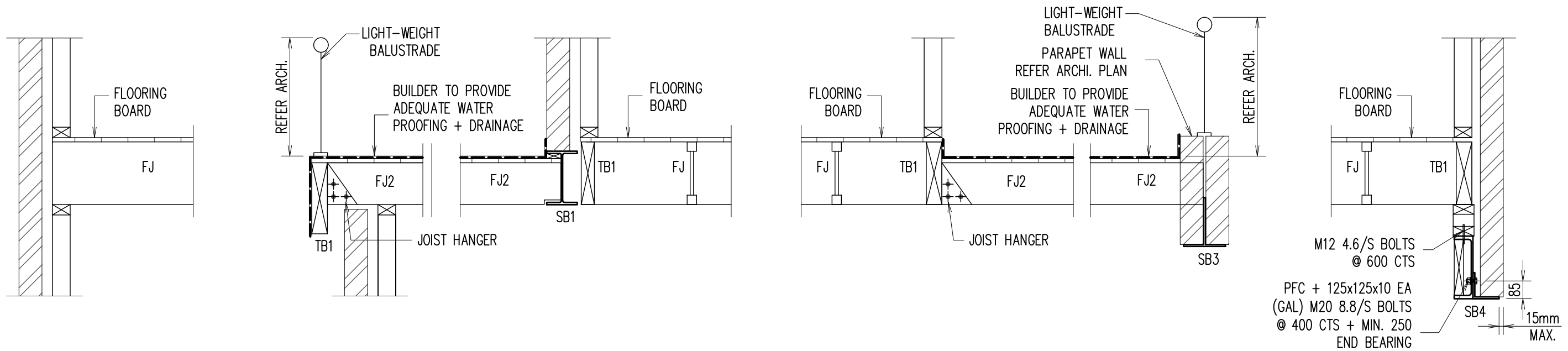
SECTION 1 SCALE 1:20
