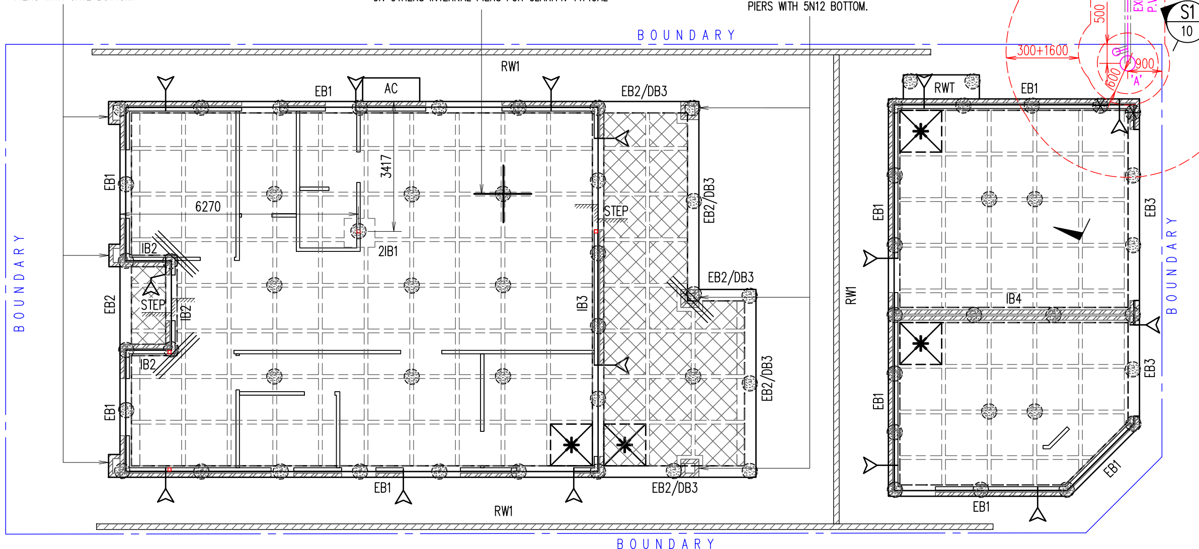
GROUND FLOOR WAFFLE SLAB LAYOUT PLAN SCALE 1:100
