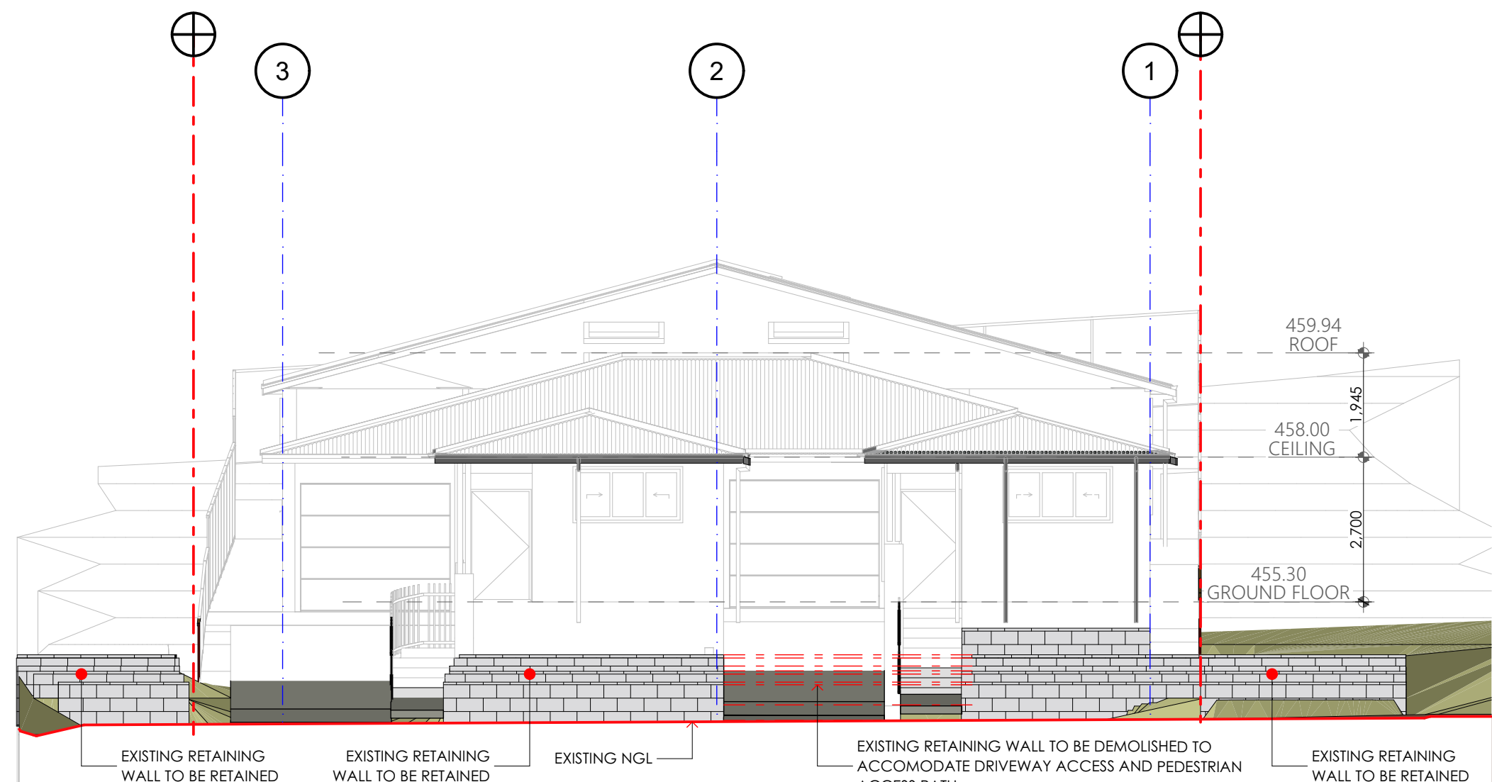
NORTH EASTERN FENCE ELEVATION 1:100
