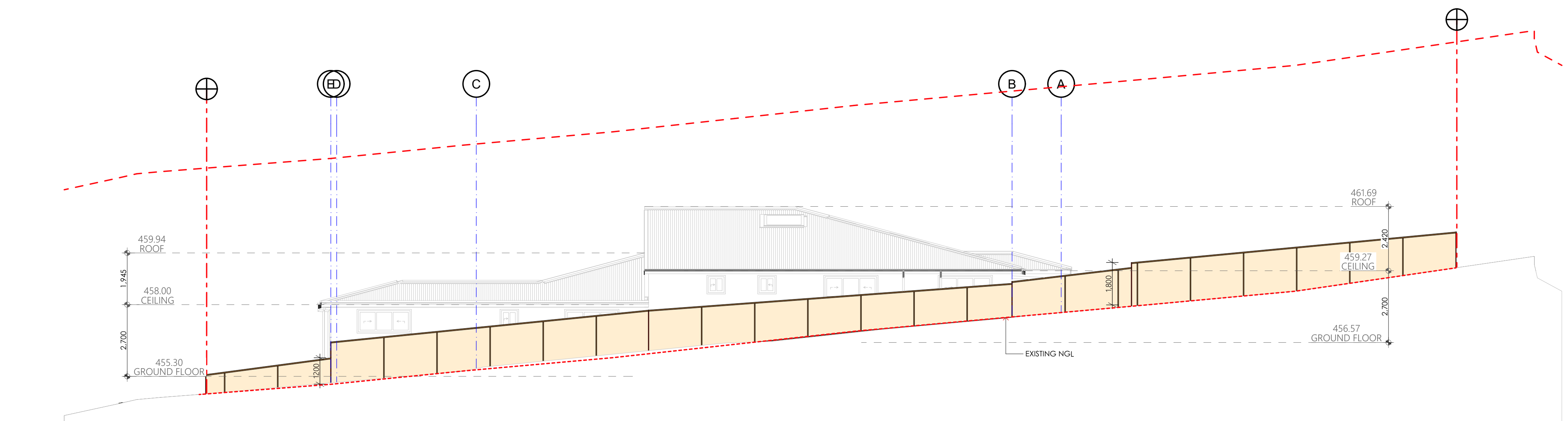
NORTH WESTERN FENCE ELEVATION 1:100
