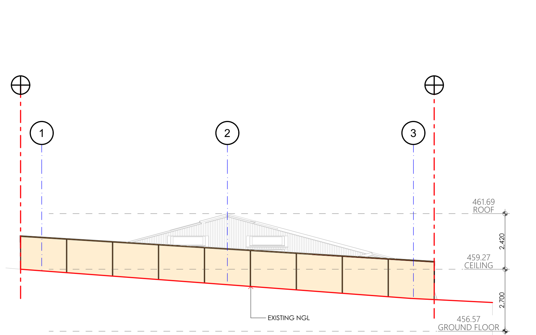
SOUTH WESTERN FENCE ELEVATION 1:100
