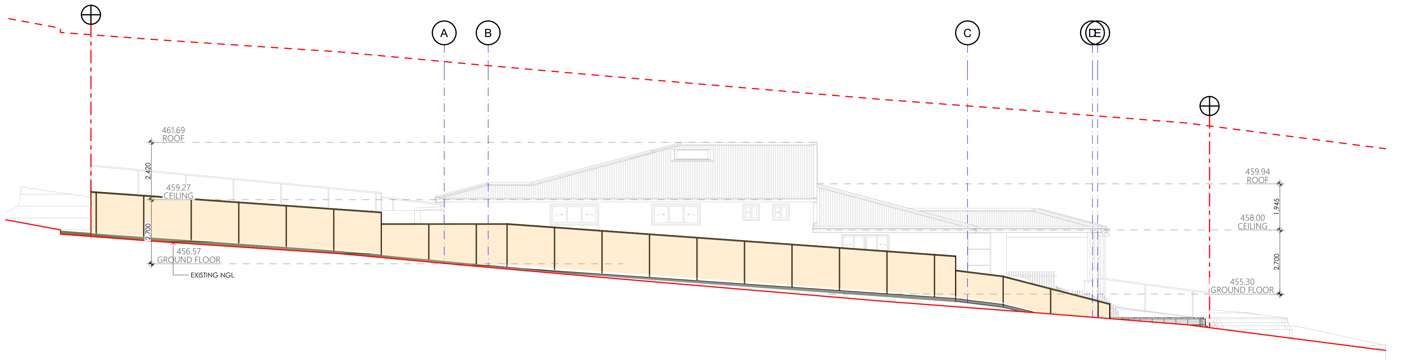
SOUTH EASTERN FENCE ELEVATION 1:100
