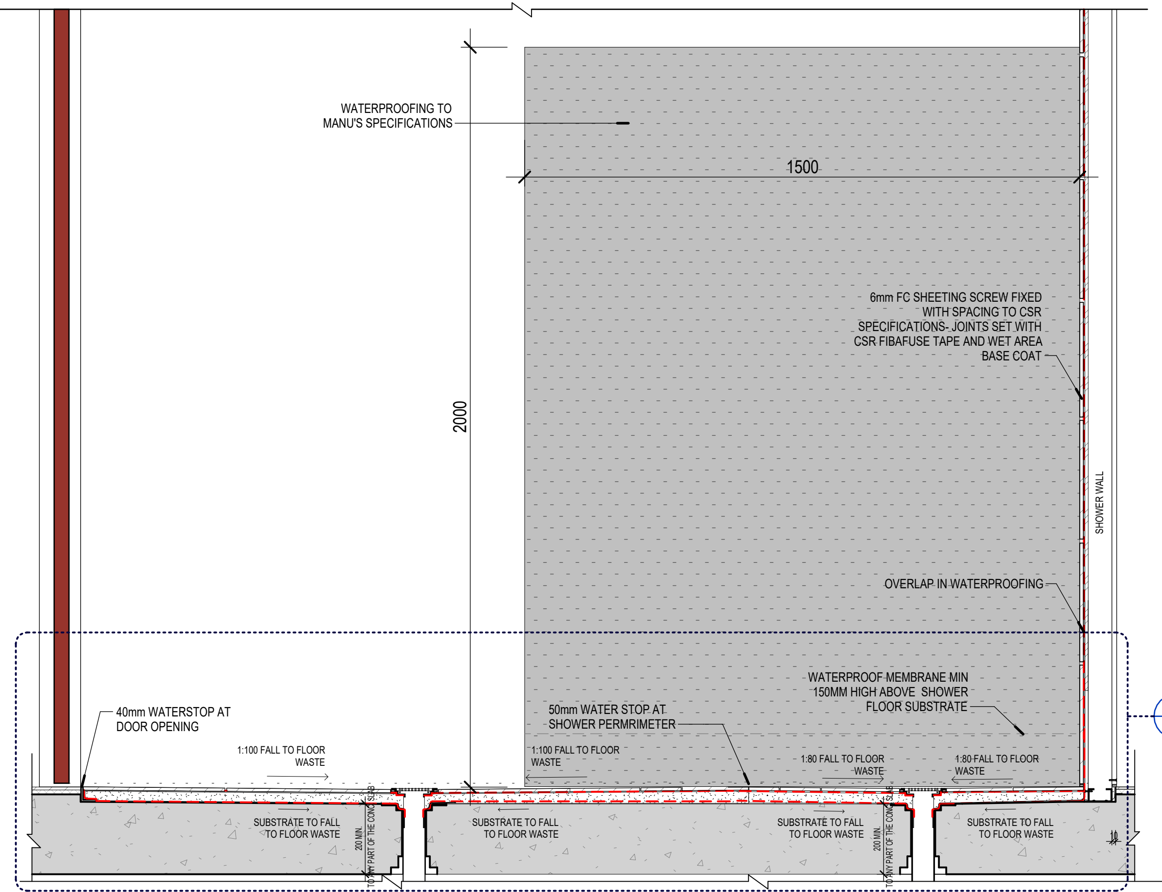
2 ENCLOSED SHOWER - SIDE VIEW 1 1: 10
