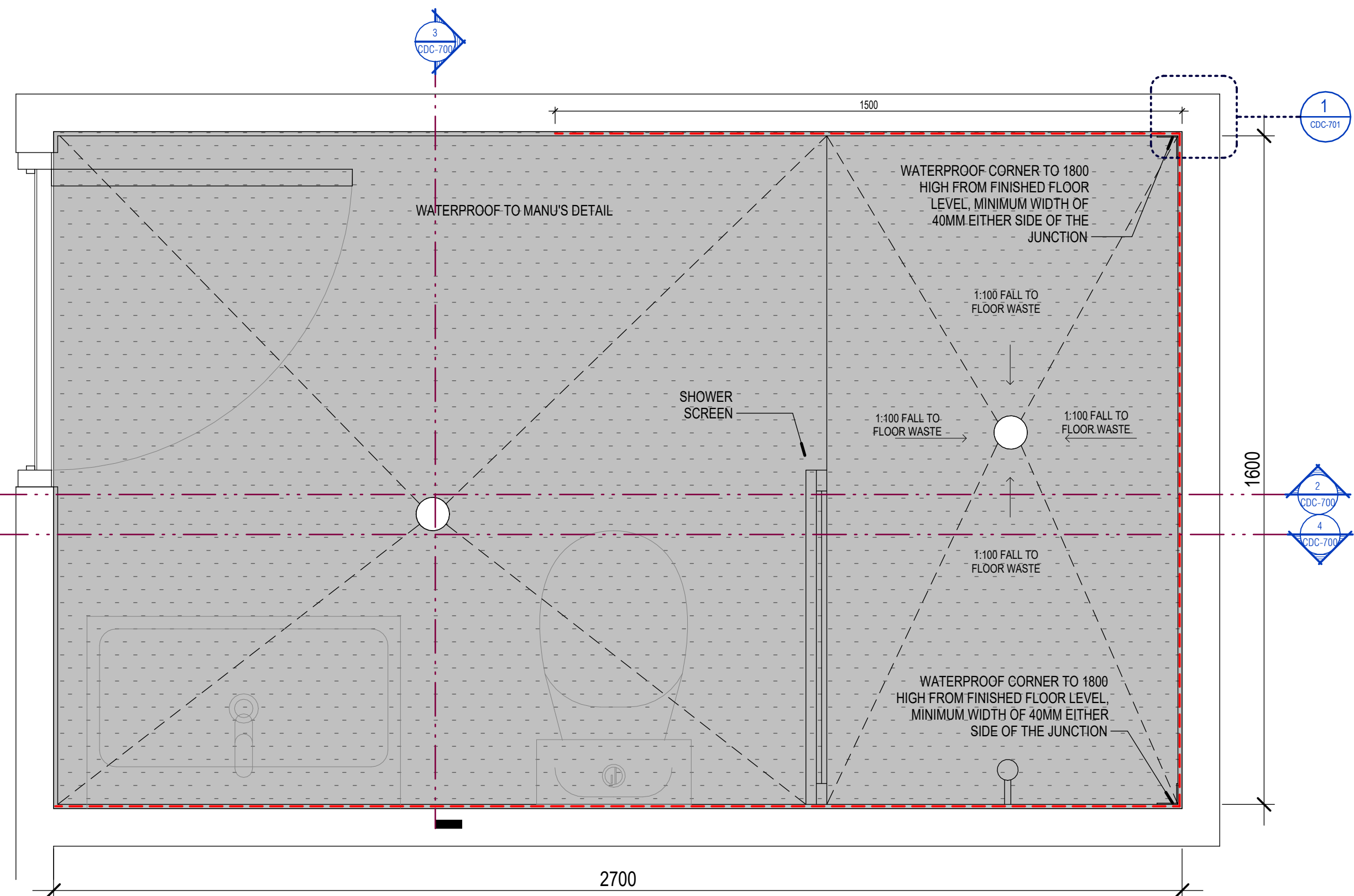
1 TYPICAL ENCLOSED SHOWER - PLAN VIEW 1: 10
