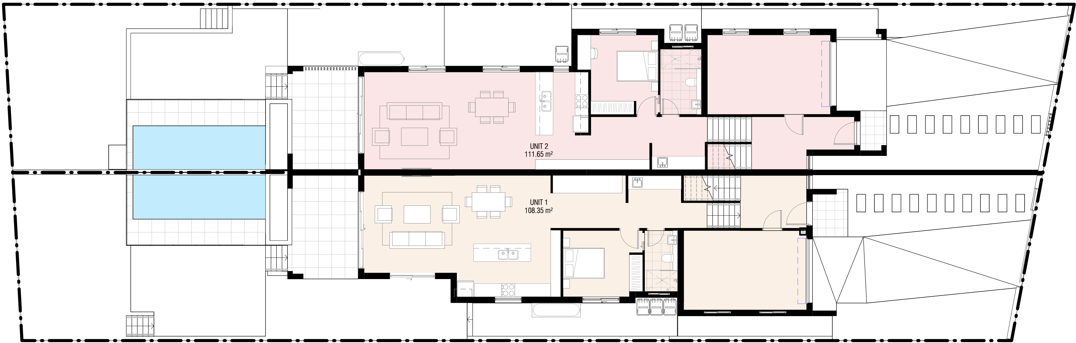
2 GROUND FLOOR PLAN 1: 100
