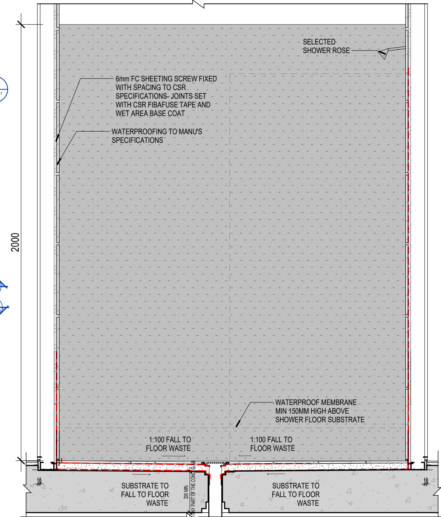
3 ENCLOSED SHOWER - FRONT VIEW 1: 10
