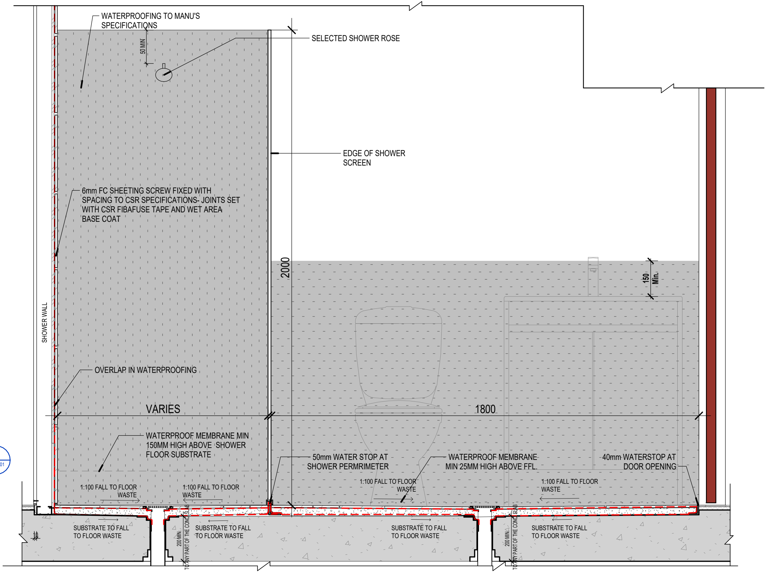
4 ENCLOSED SHOWER - SIDE VIEW 2 1: 10
