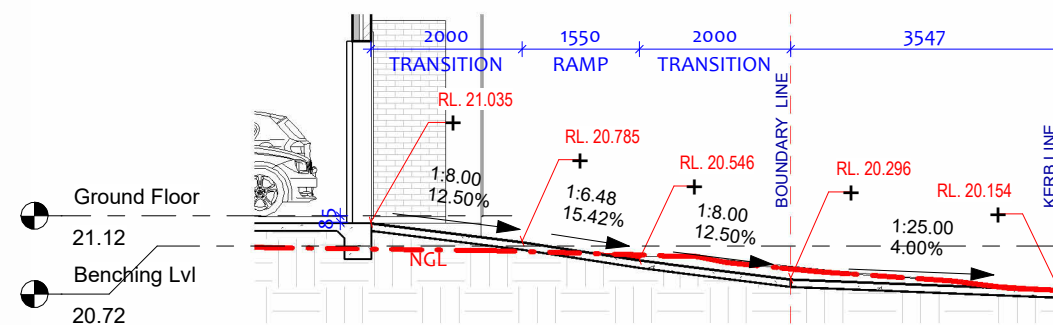
2 DRIVEWAY SECTION 1 : 100
