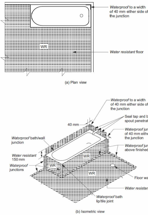
Figure 10.2.4b: Areas adjacent to baths and spas without showers for timber floors including particle-board, plywood and other floor materials
