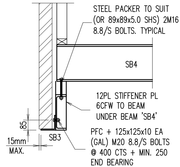
DETAIL – C SCALE 1:20
