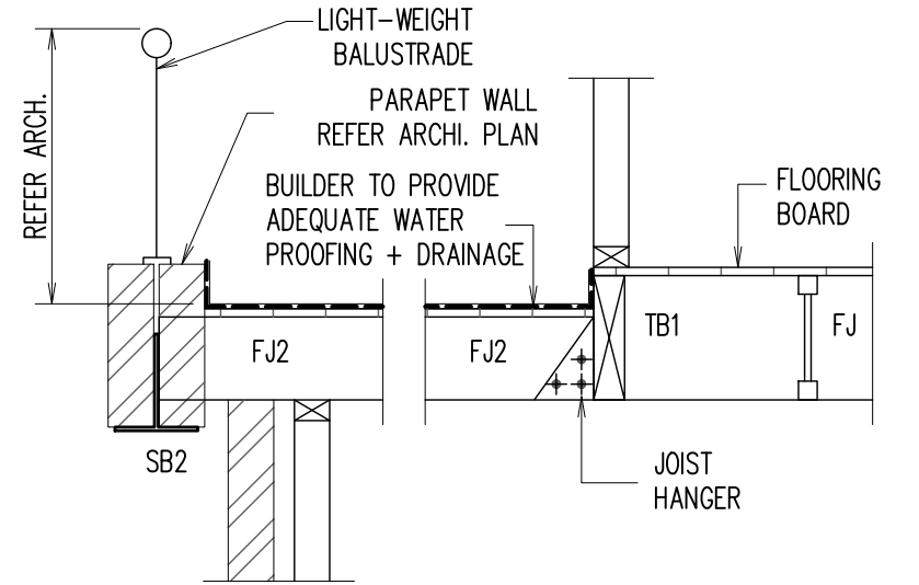
SECTION 4 SCALE 1:20
