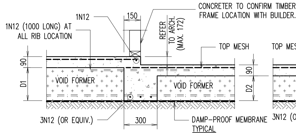
TYPICAL EDGE BEAM – 'EB1' ALTERNATIVELY REFER TO 'DB1' FOR DETAILS
