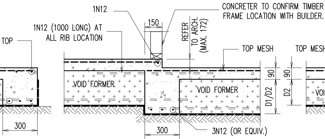
INTERNAL STEPDOWN BEAM – 'IB3' ALTERNATIVELY REFER TO 'DB2' FOR DETAILS
