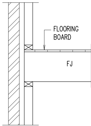
SECTION 1 SCALE 1:20
