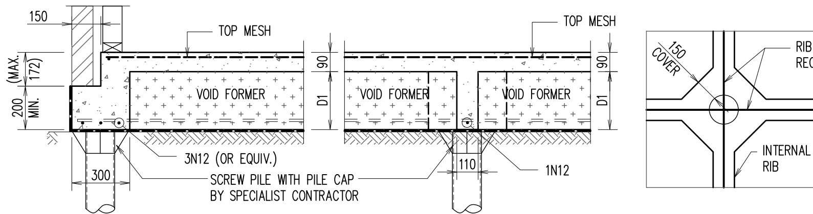
TYPICAL SLAB TO SCREW PILE CONNECTION DETAILS – OPTION 2
