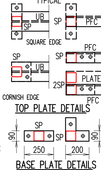
TYPICAL POST TO SLAB DETAIL
