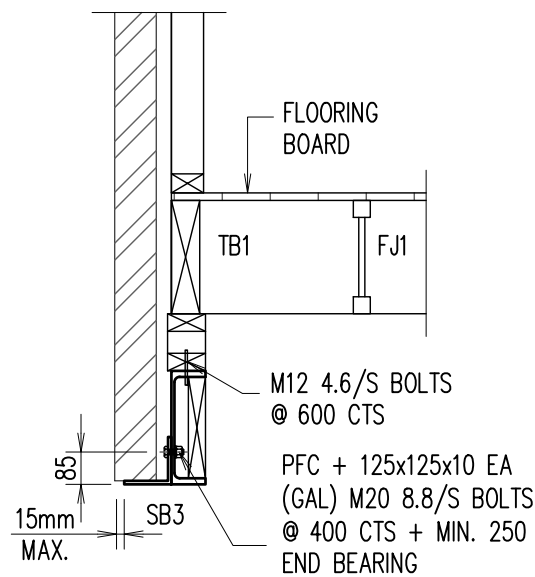
SECTION 5 SCALE 1:20
