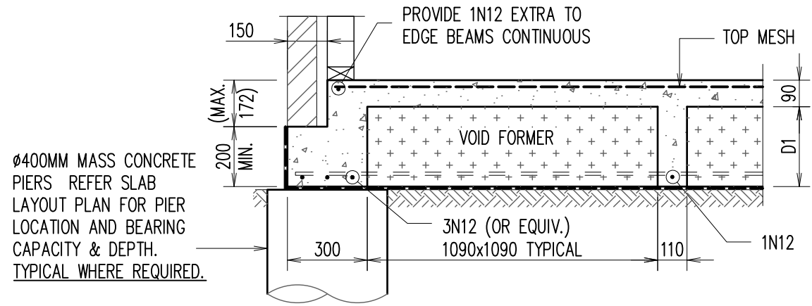
TYPICAL EDGE BEAM – 'EB1' ALTERNATIVELY REFER TO 'DB1' FOR DETAILS
