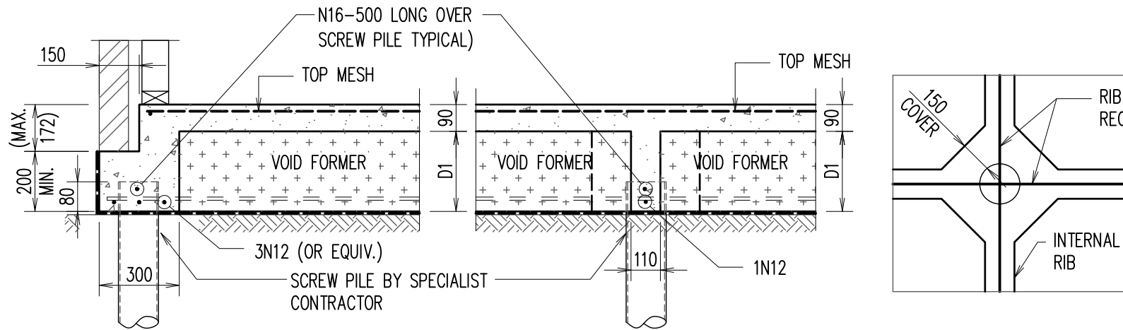
TYPICAL SLAB TO SCREW PILE CONNECTION DETAILS – OPTION 1
