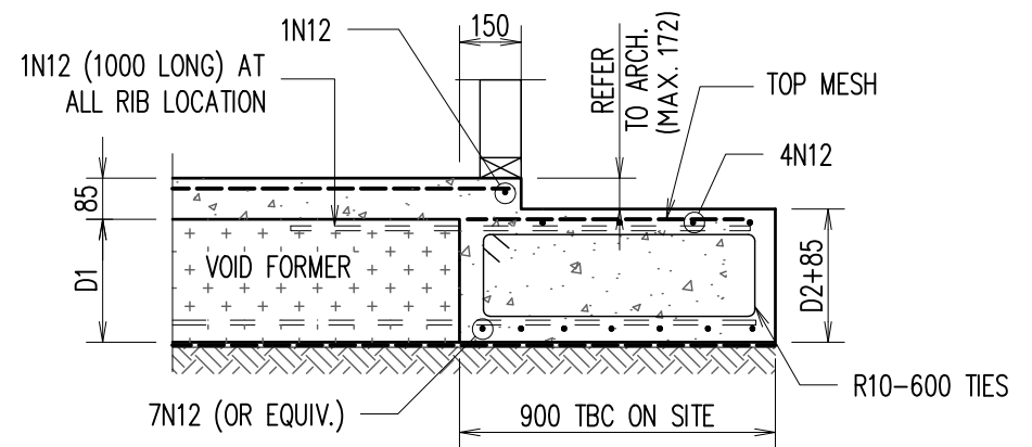
FRONT PORCH BEAM – 'EB5'
