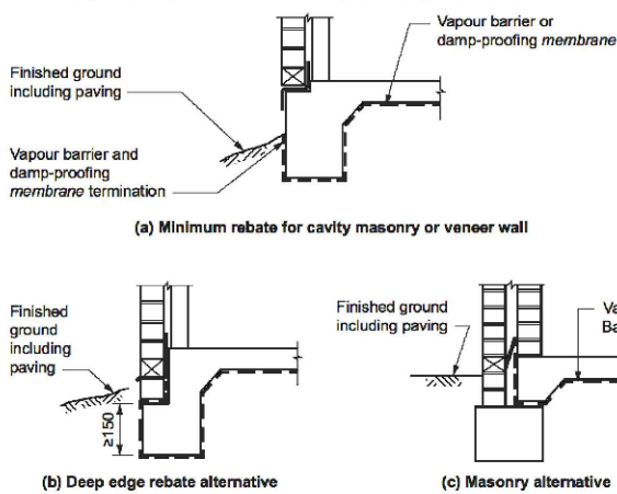
Figure 4.2.8: Acceptable vapour barrier and damp-proofing membrane location
