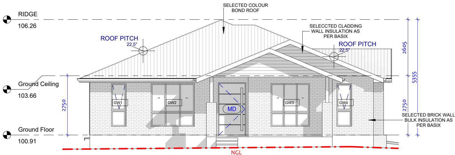
1 North-West Elevation 1 : 100
