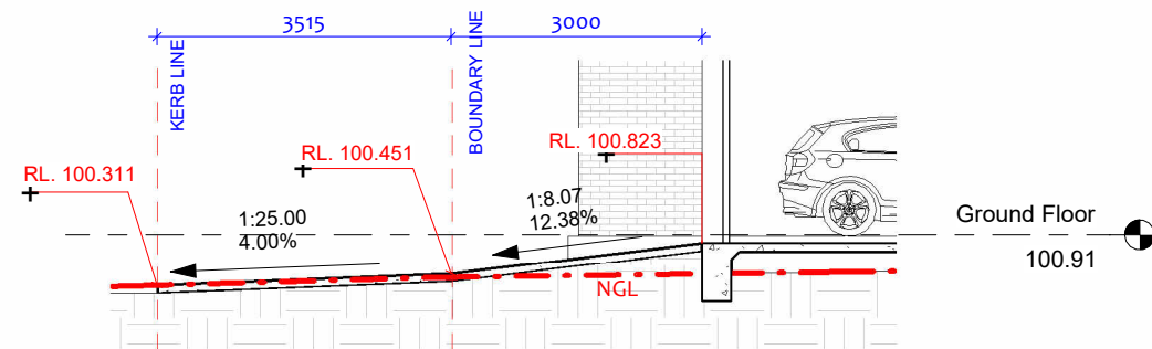
2 DRIVEWAY SECTION 1 : 100
