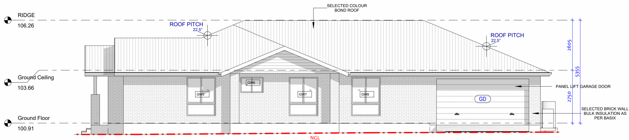
2 South-West Elevation 1 : 100
