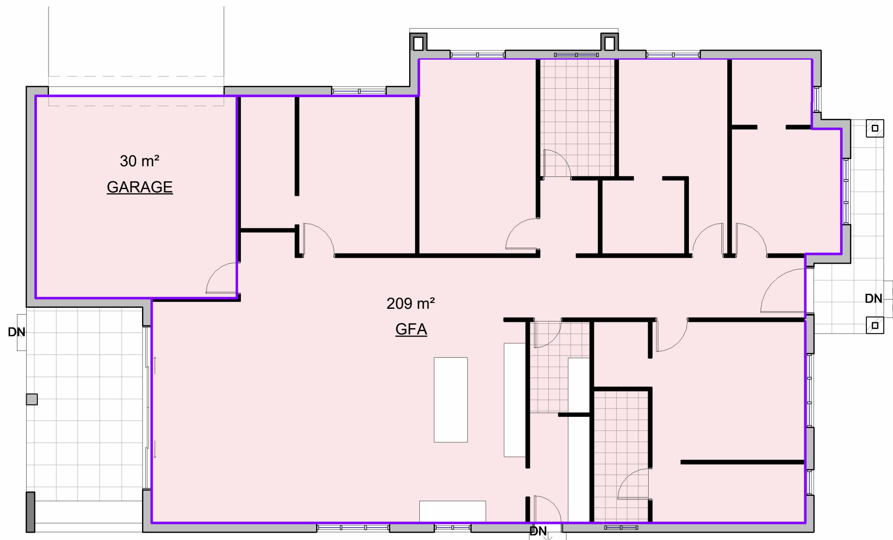
1 Ground Floor 1 : 100
