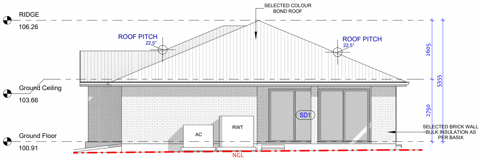
2 South-East Elevation 1 : 100
