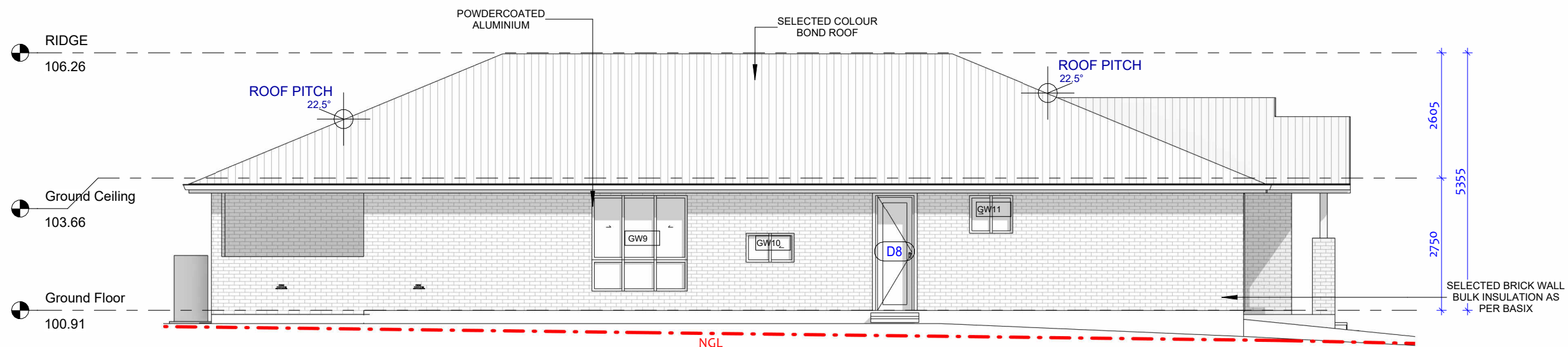
1 North-East Elevation 1 : 100
