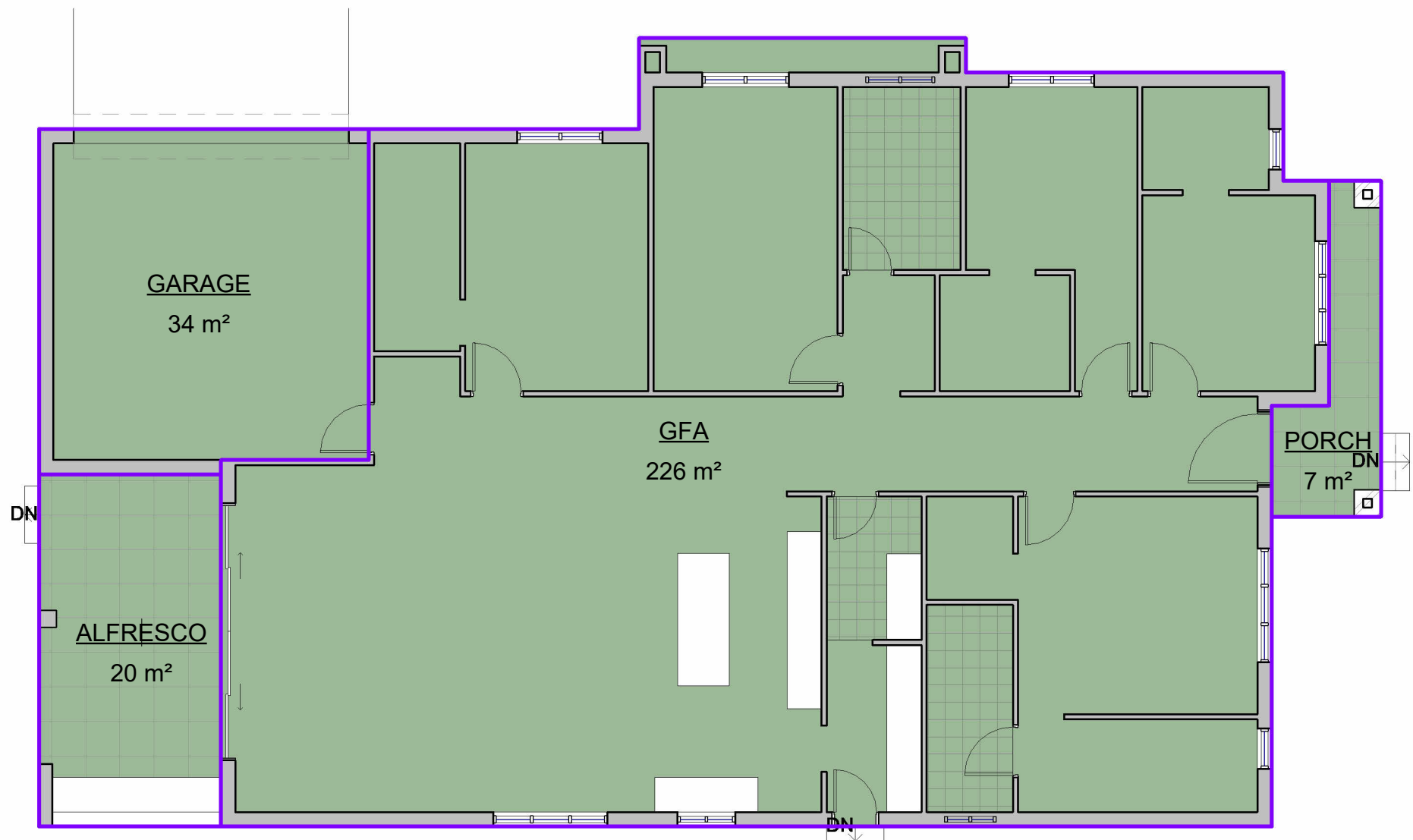
1 Ground Floor 1 : 100
