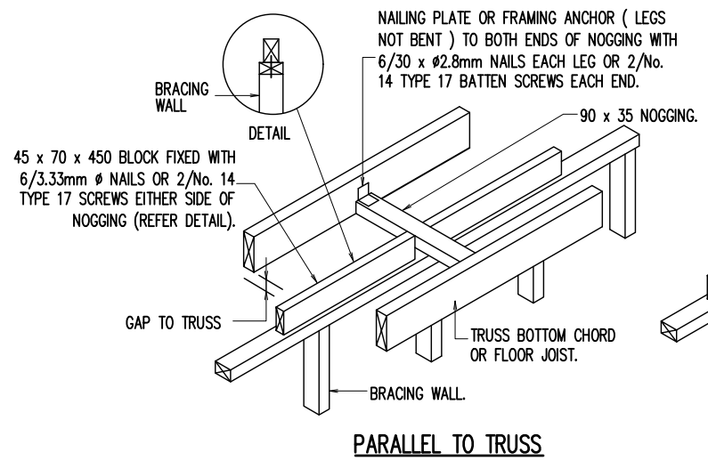
TIMBER BRACING WALL TOP CONNECTION DETAIL
