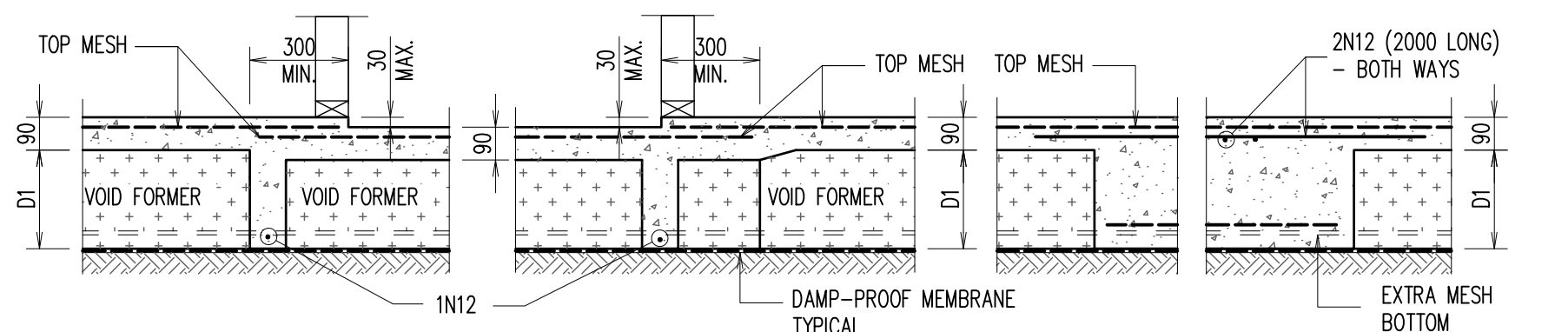
TYPICAL WET AREA STEP DETAIL
