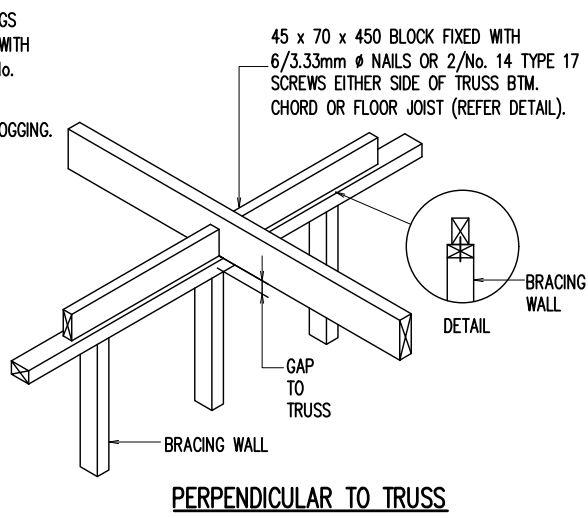
TIMBER BRACING WALL TOP CONNECTION DETAIL
