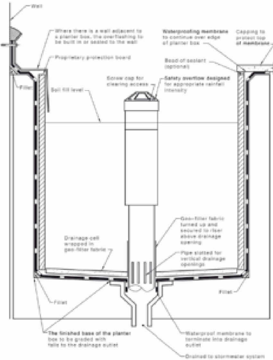
FIGURE 2.17 TYPICAL PLANTER BOX CONSTRUCTION
