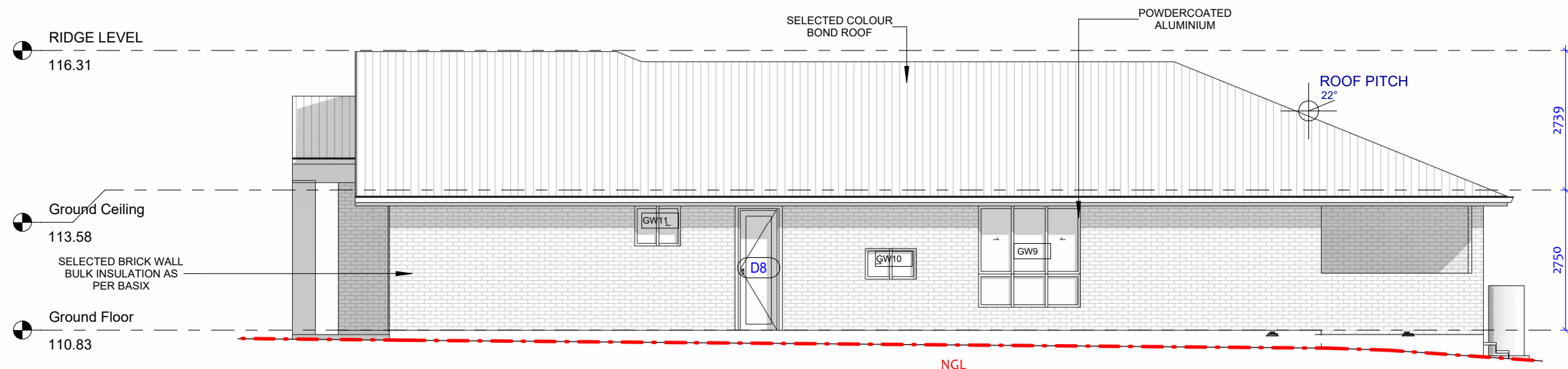
1 NORTH Elevation 1 : 100
