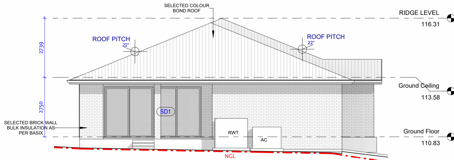
2 WEST Elevation 1 : 100
