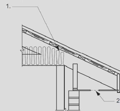
Figure 10.8.3 (explanatory): Example of roof space with low level ventilation
