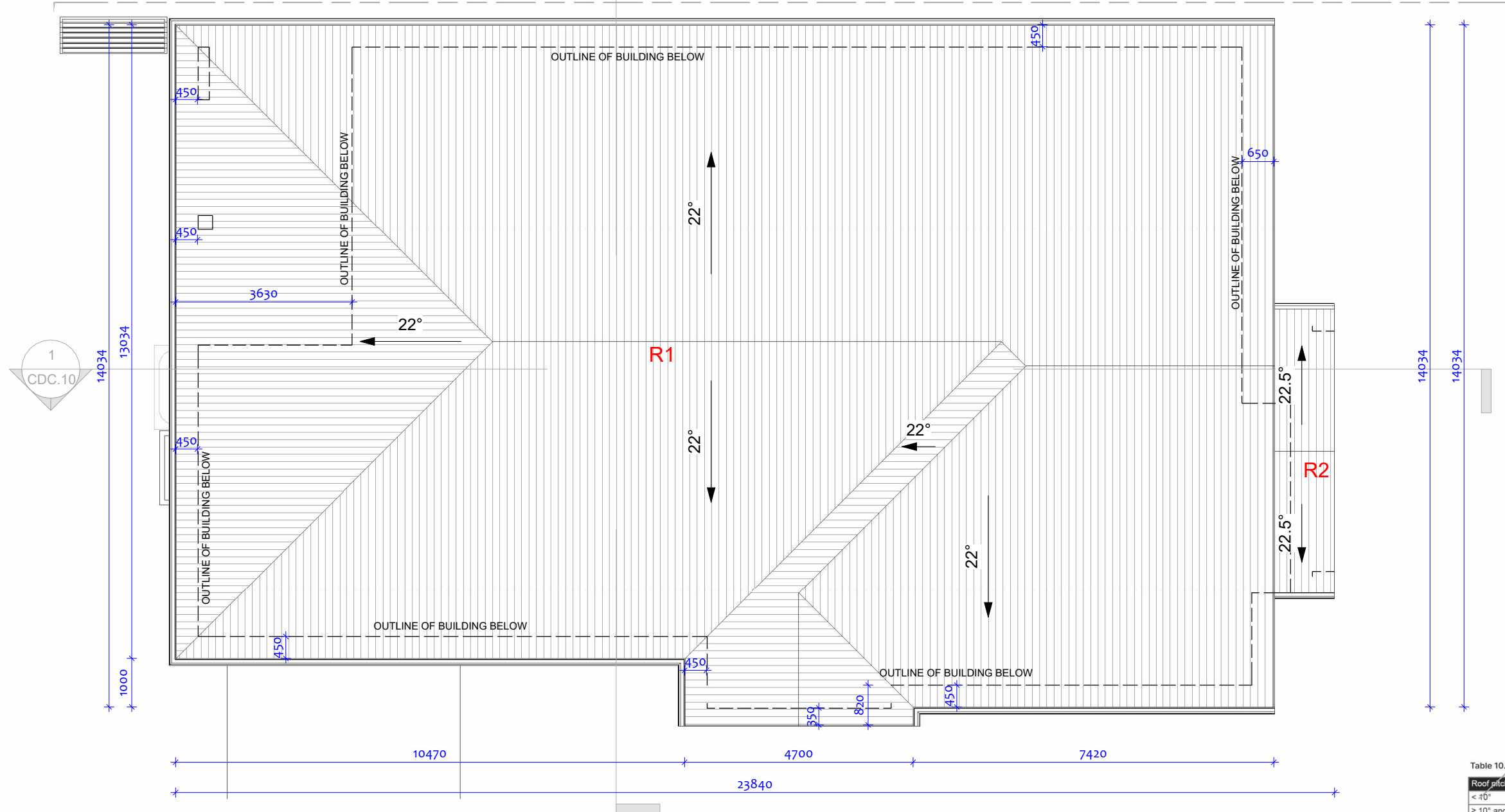
Figure 10.8.3 (explanatory): Example of roof space with low level ventilation
