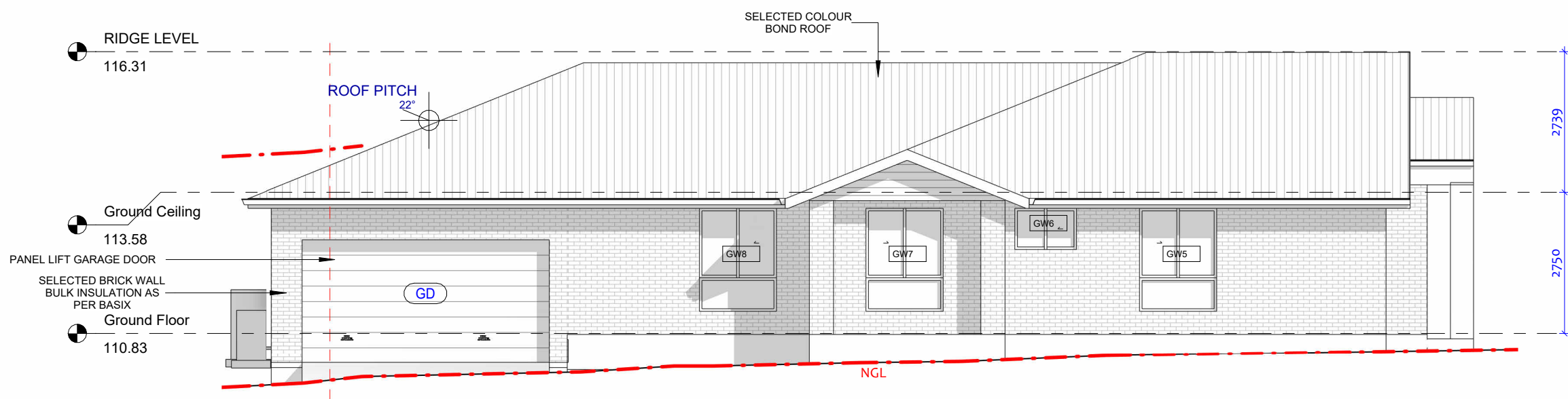
2 SOUTH Elevation 1 : 100
