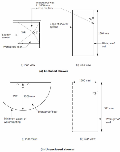
Figure Notes Wall/floor junction heights are to be as per 10.2.2 to 10.2.6 (as applicable).
