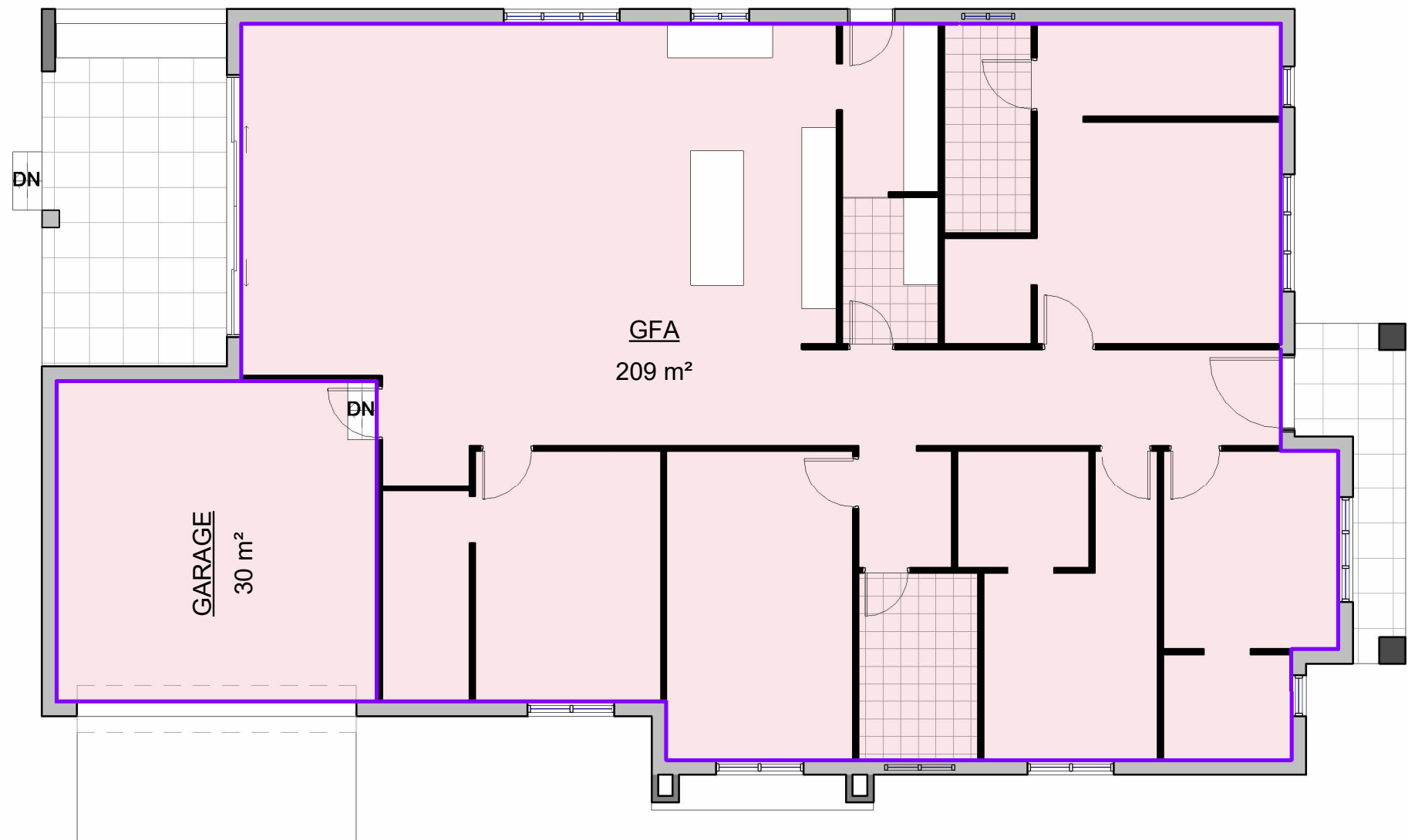
1 Ground Floor 1 : 100
