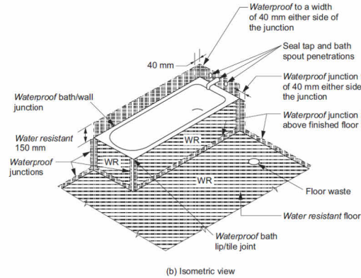
Figure 10.2.4b: Areas adjacent to baths and spas without showers for timber floors including particle-board, plywood and other floor materials
