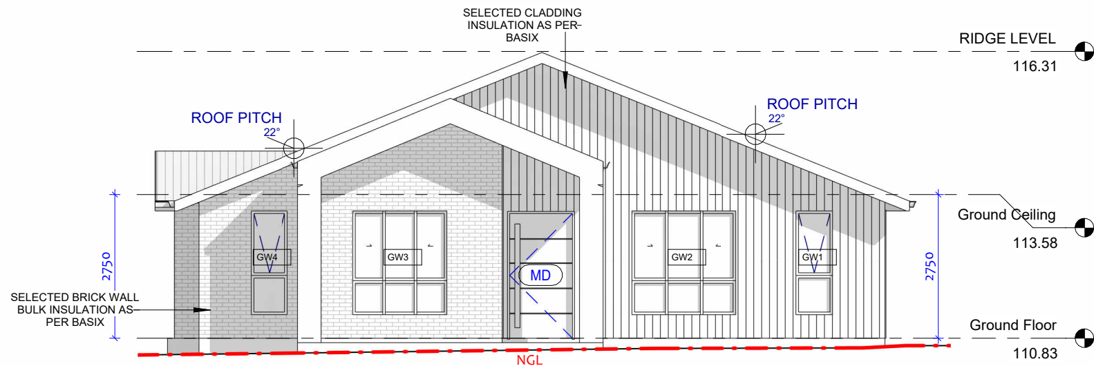
1 EAST Elevation 1 : 100
