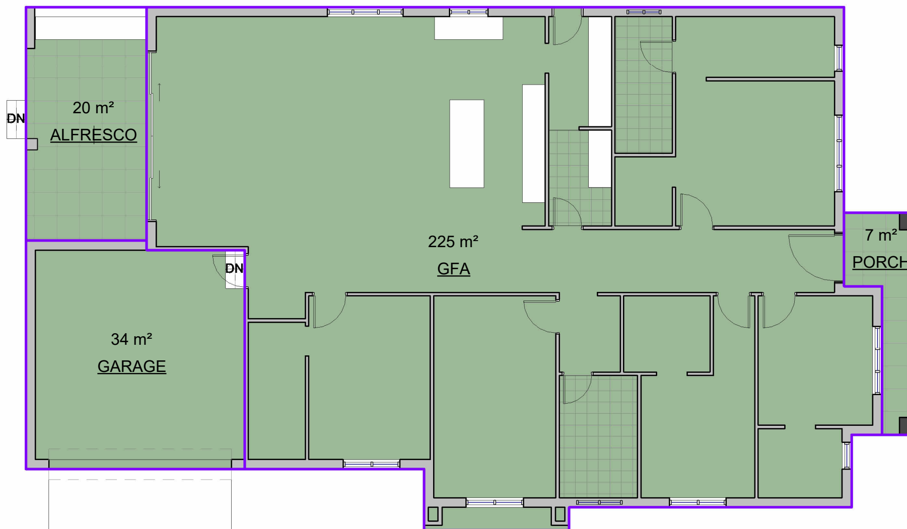
1 Ground Floor 1 : 100
