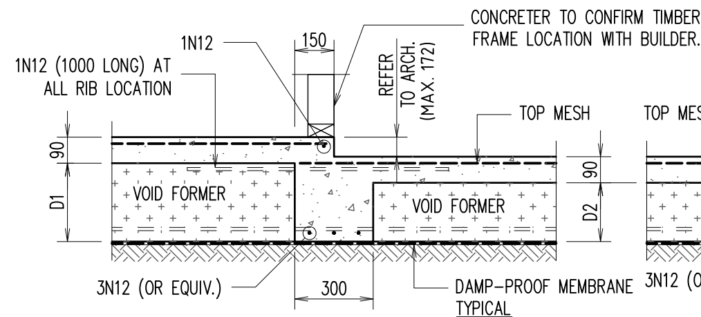
INTERNAL STEPDOWN BEAM – 'IB2'
