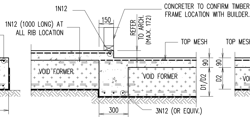
INTERNAL STEPDOWN BEAM – 'IB3'
