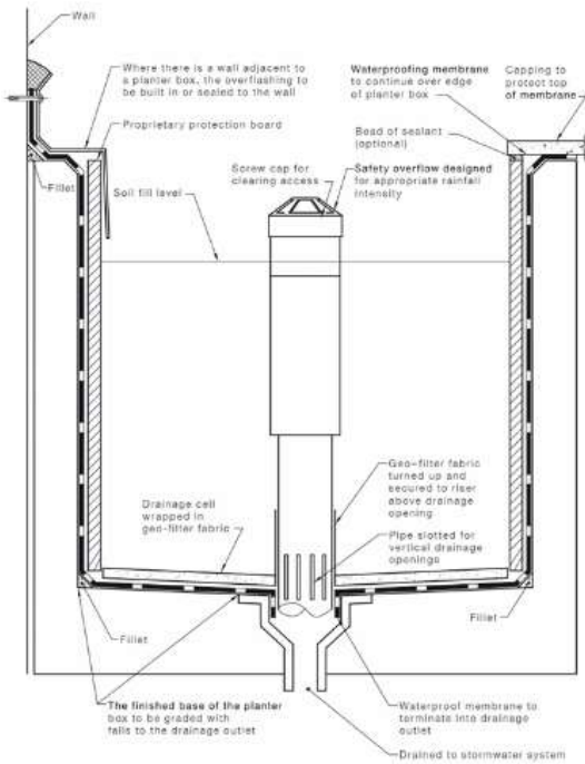
FIGURE 2.17 TYPICAL PLANTER BOX CONSTRUCTION
