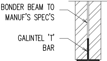
DETAIL - A SCALE 1:20
