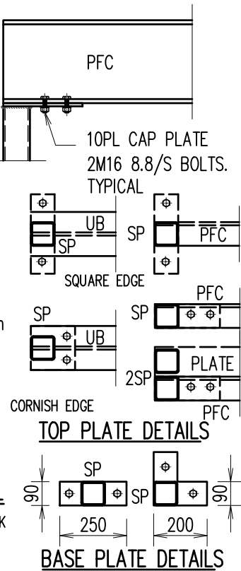
TYPICAL POST TO SLAB DETAIL
