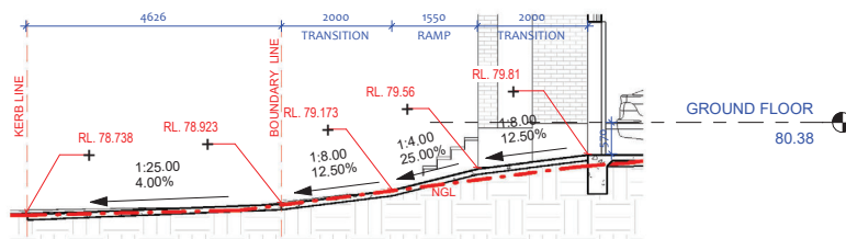
2 DRIVEWAY SECTION 1 : 100
