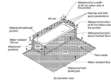
Figure 10.2.4b: Areas adjacent to baths and spas without showers for timber floors including particle-board, plywood and other floor materials
