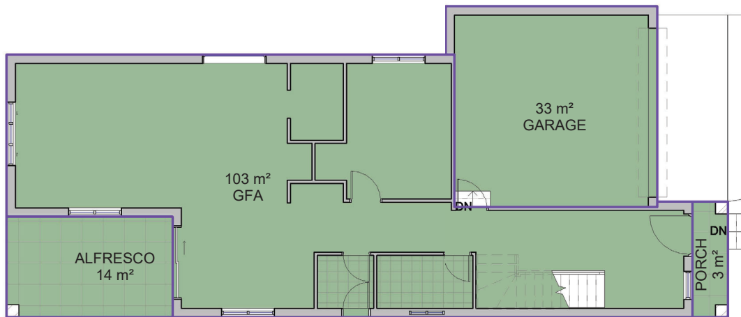
1 GROUND FLOOR 1 : 100
