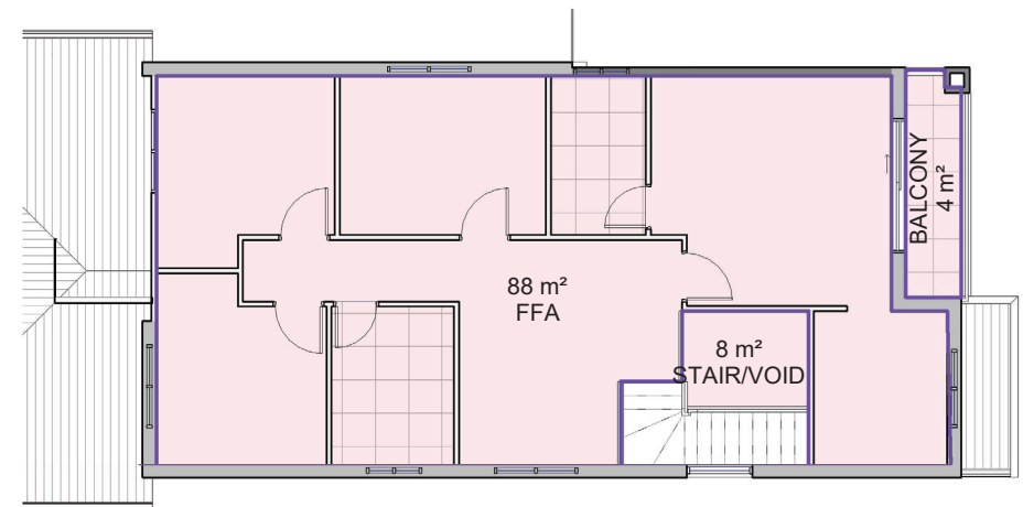
2 FIRST FLOOR 1 : 100
