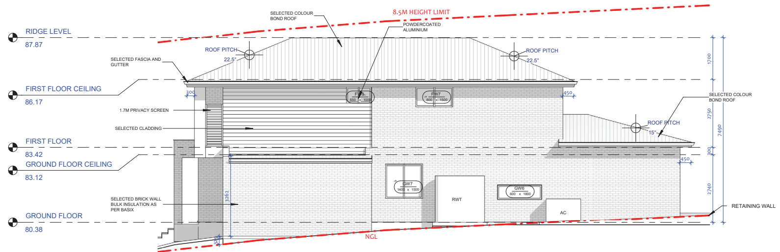
2 EAST ELEVATION 1 : 100
