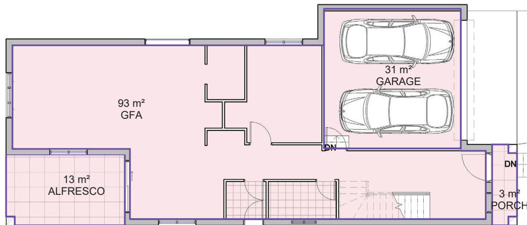
1 GROUND FLOOR 1 : 100
