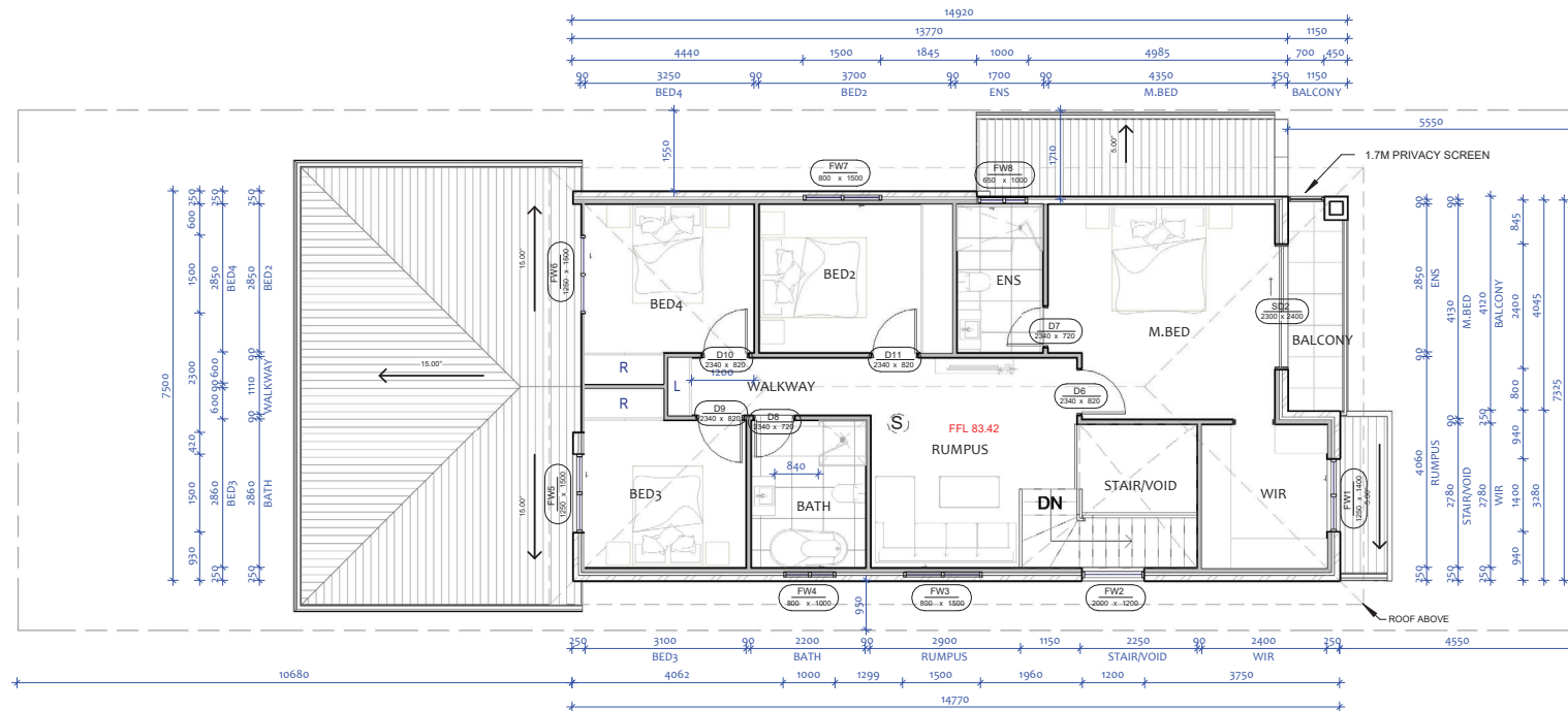
1 FIRST FLOOR PLAN 1 : 100
