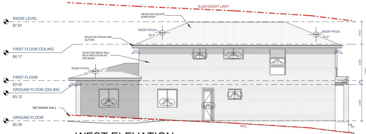
1 WEST ELEVATION 1 : 100
