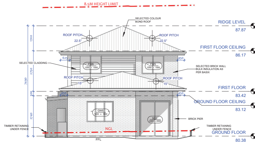
1 NORTH ELEVATION 1 : 100
