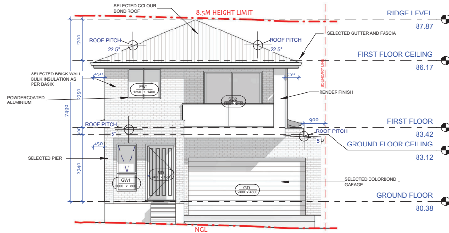
2 SOUTH ELEVATION 1 : 100
