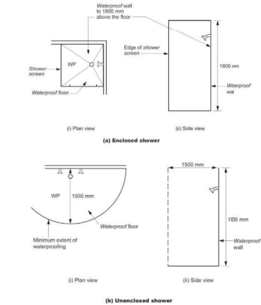
Figure Notes Wall/floor junction heights are to be as per 10.2.2 to 10.2.6 (as applicable).
