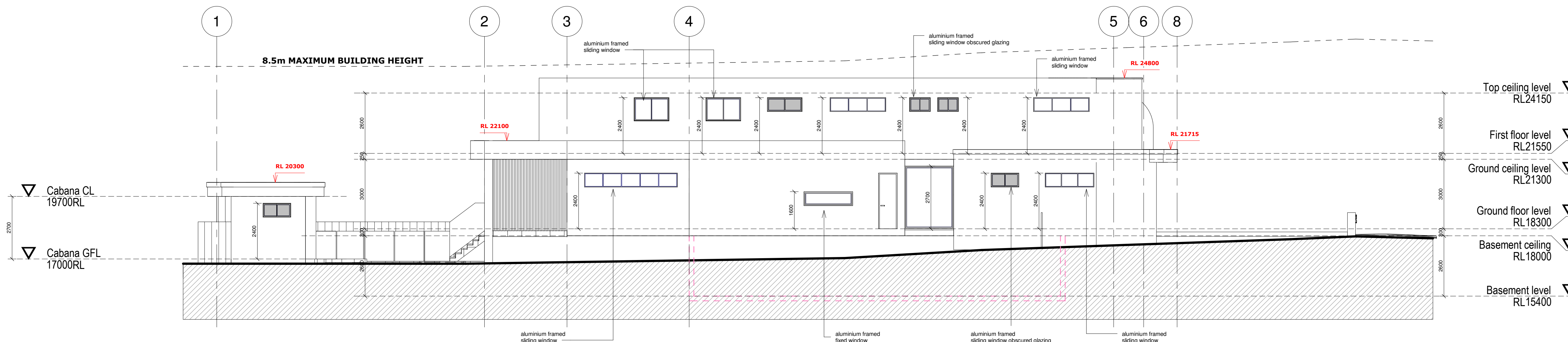
3 North elevation 1 : 100
