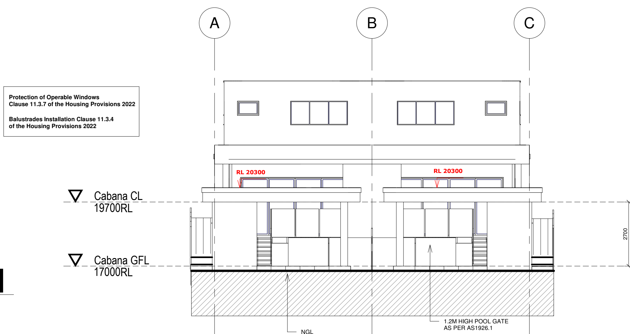
4 West Elevation 1 1:100
