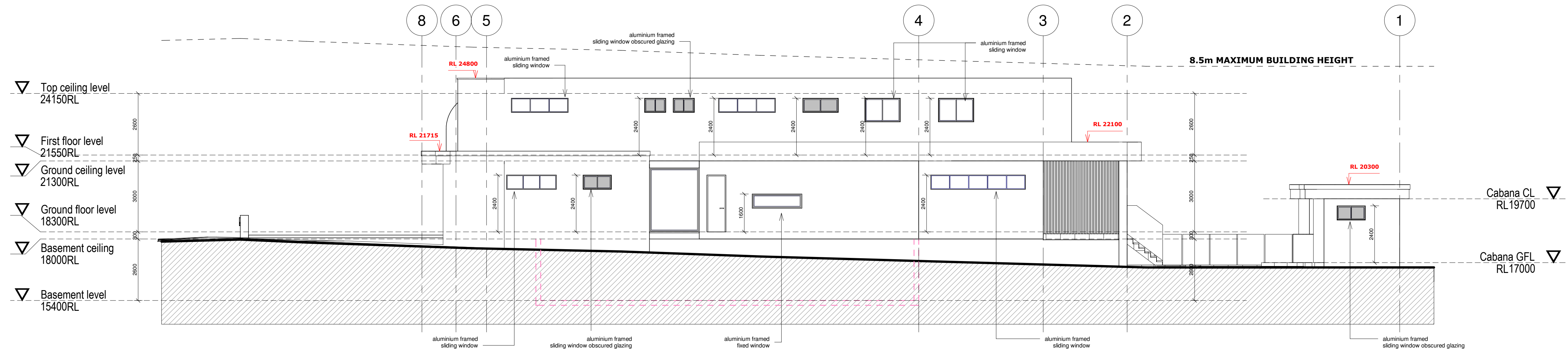
1 South elevation 1:100
