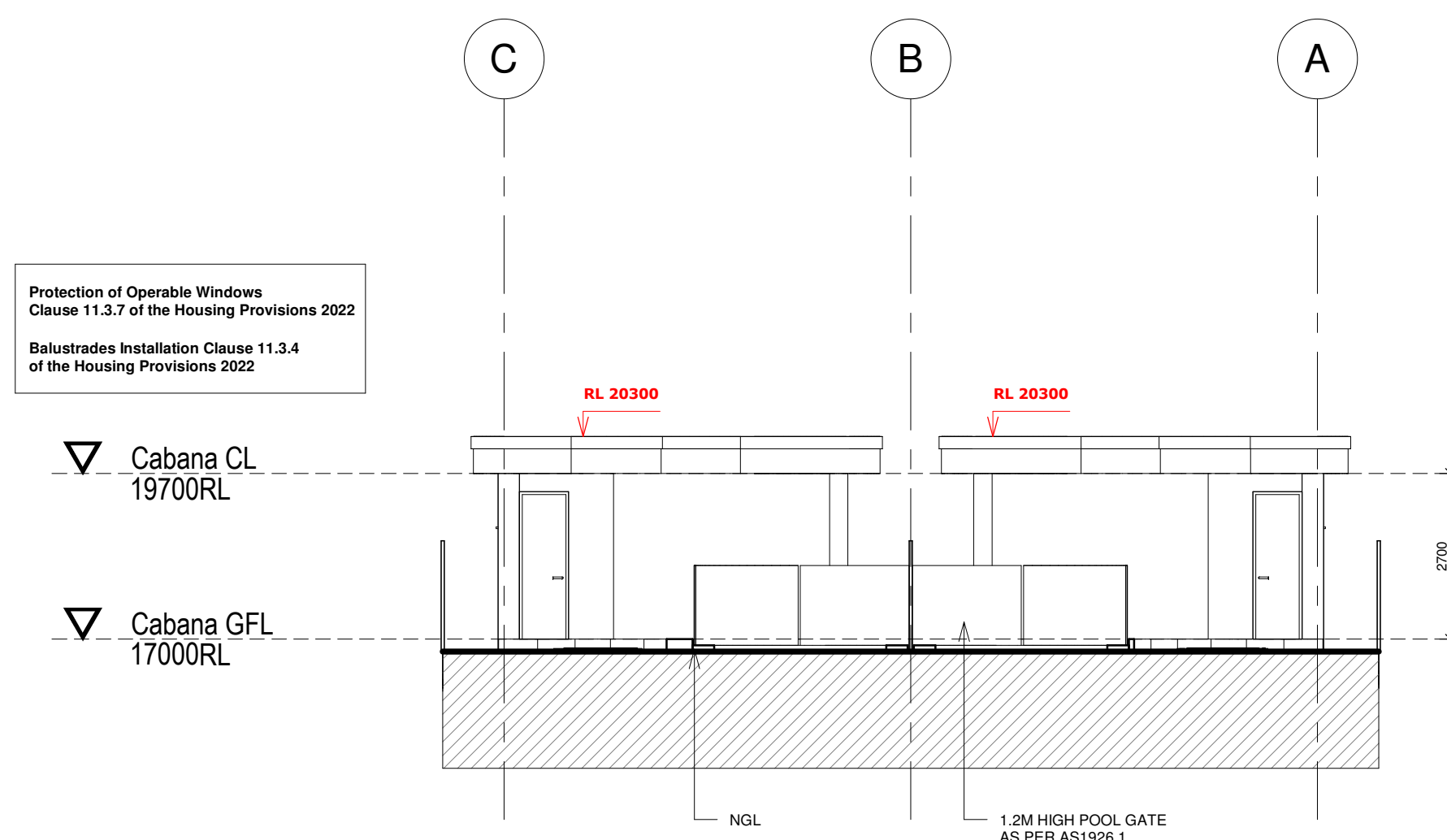
3 East Elevation 1 1:100
