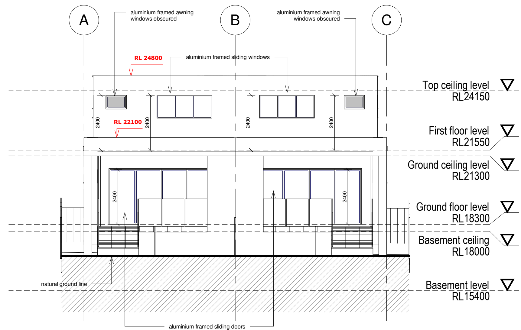
2 West elevation 1 : 100
