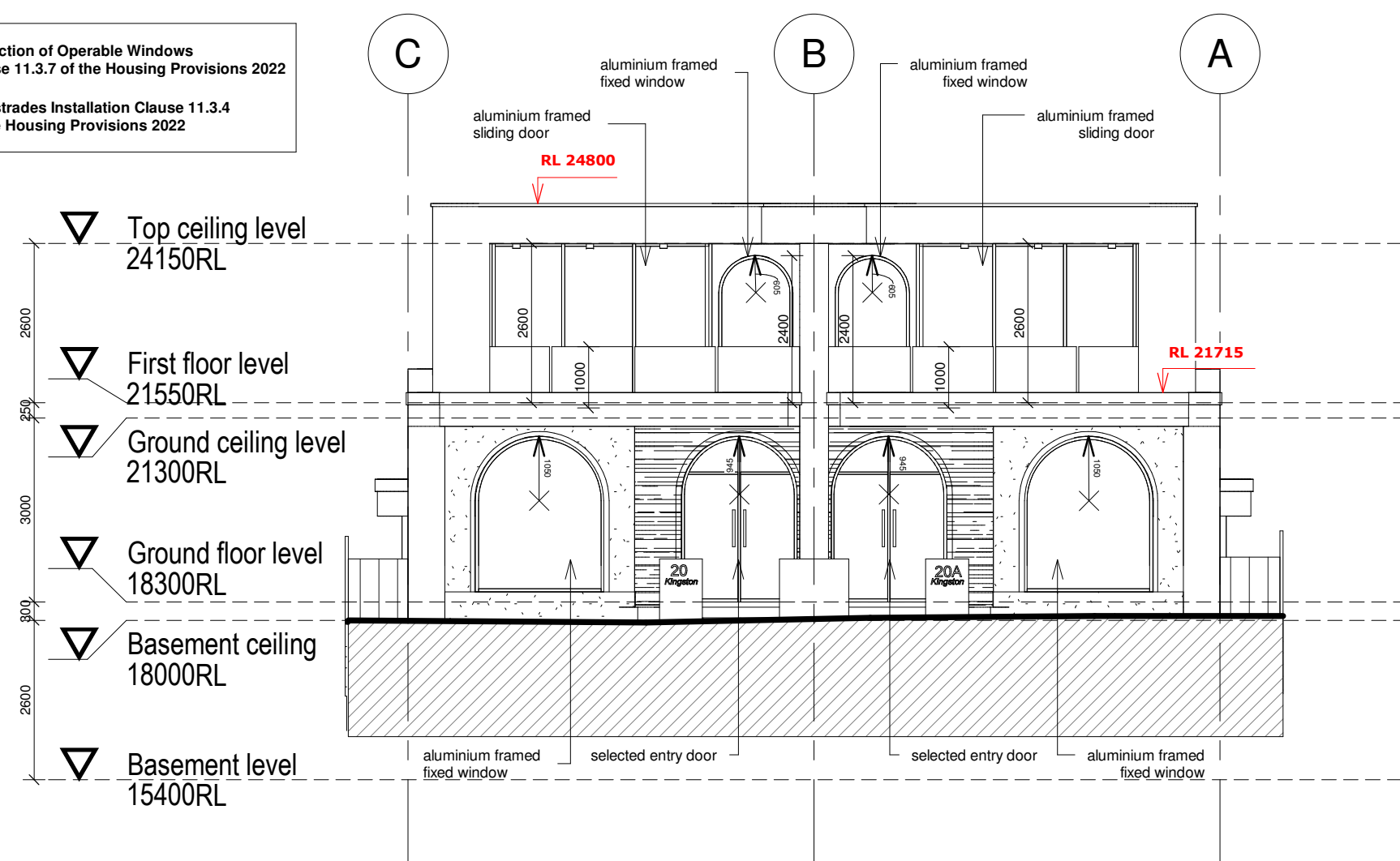
1 East elevation 1 : 100
