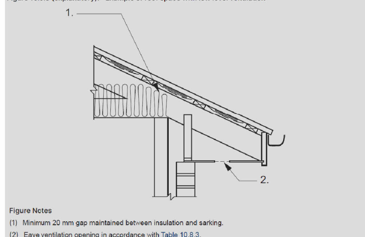
Figure 10.8.3 (explanatory): Example of roof space with low level ventilation
