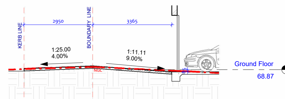
1 DRIVEWAY SECTION 1 : 100
