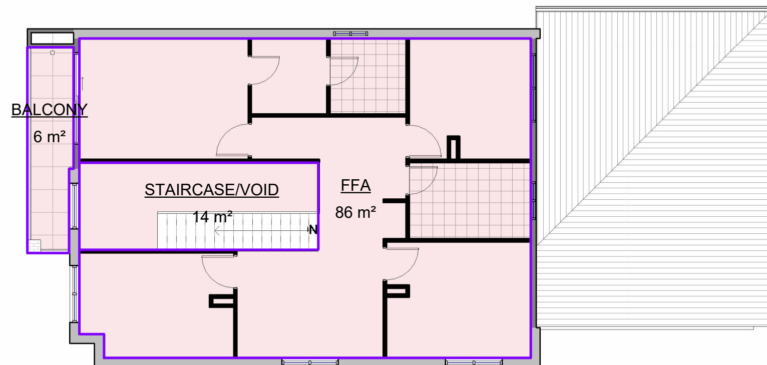
2 First Floor 1 : 100
