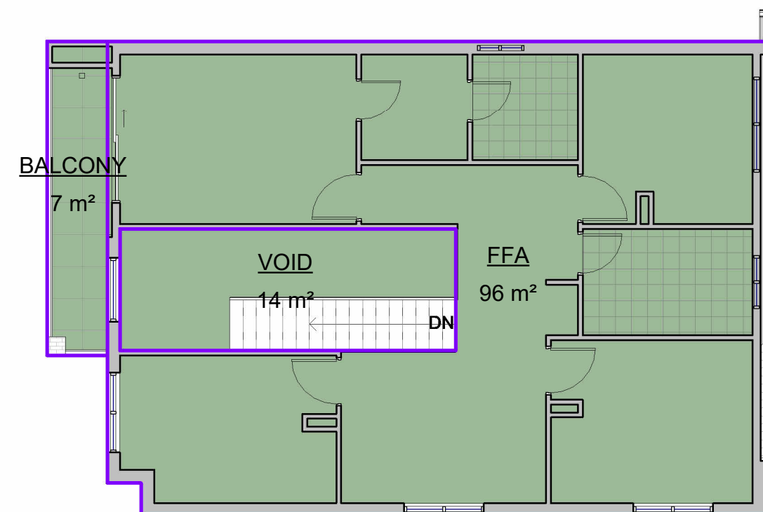
2 First Floor 1 : 100
