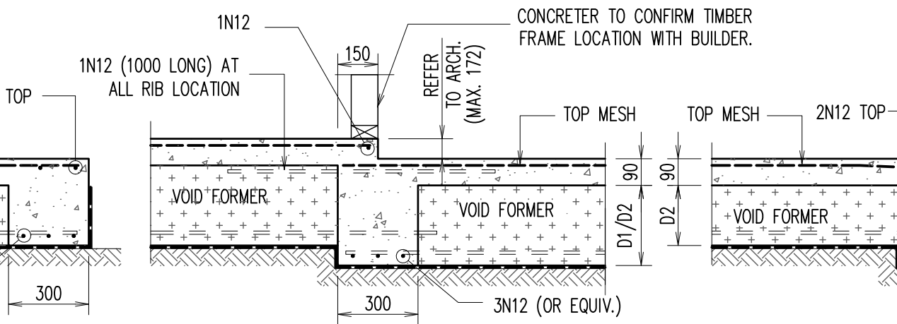
INTERNAL STEPDOWN BEAM – 'IB3' ALTERNATIVELY REFER TO 'DB2' FOR DETAILS
