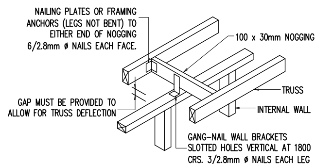
NON LOAD BEARING WALL PARALLEL TO TRUSSES
