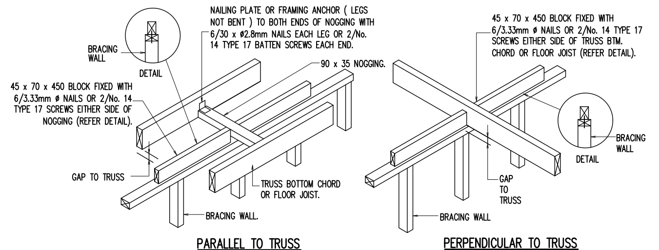
TIMBER BRACING WALL TOP CONNECTION DETAIL
