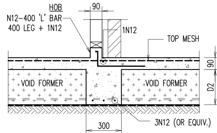
INTERNAL STEPDOWN BEAM – 'IB3' ALTERNATIVELY REFER TO 'DB2' FOR DETAILS
