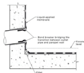
(a) Overflow through parapet
