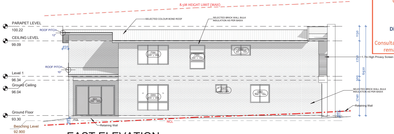
1 EAST ELEVATION 1 : 100
