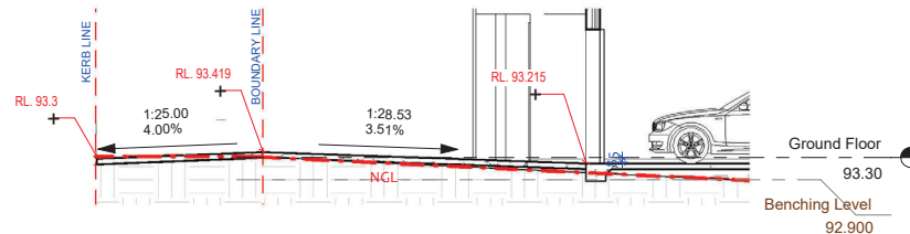
2 DRIVEWAY SECTION 1 : 100
