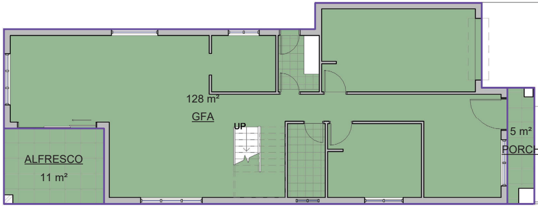
1 Ground Floor 1 : 100
