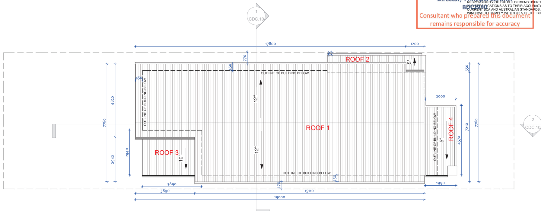
1 ROOF PLAN
