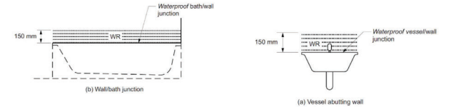
Figure 10.2.5: Bath and vessel abutting wall - areas to be protected
