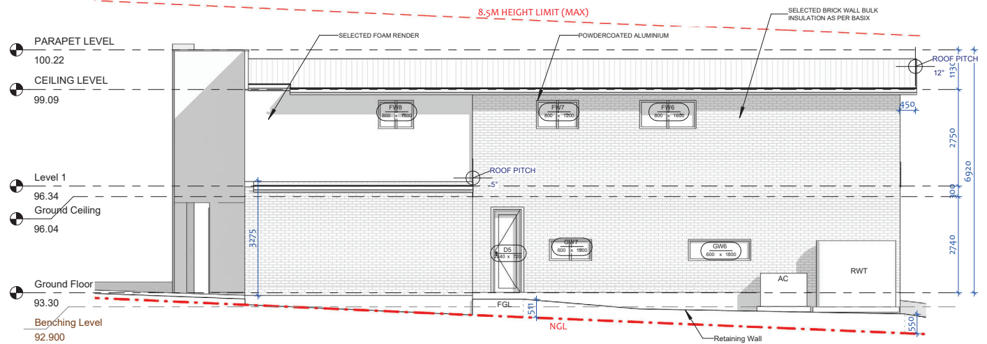
2 WEST ELEVATION 1 : 100
