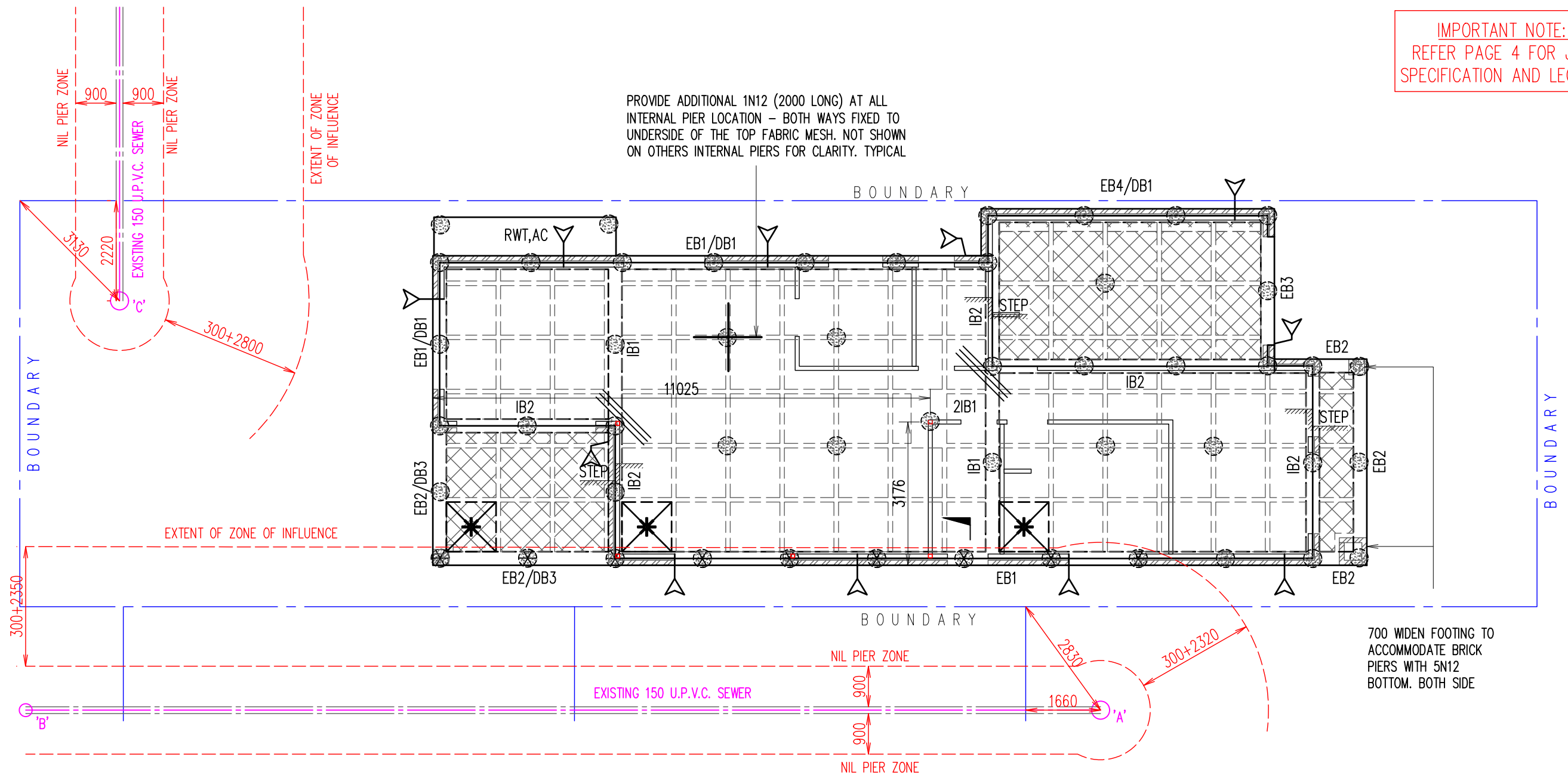
GROUND FLOOR WAFFLE SLAB LAYOUT PLAN SCALE 1:100
