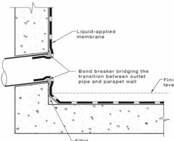
(a) Overflow through parapet
