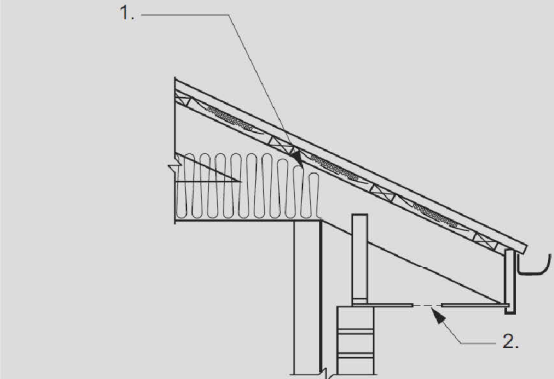
Figure 10.8.3 (explanatory): Example of roof space with low level ventilation
