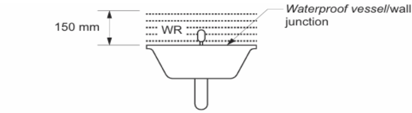
(a) Vessel abutting wall
