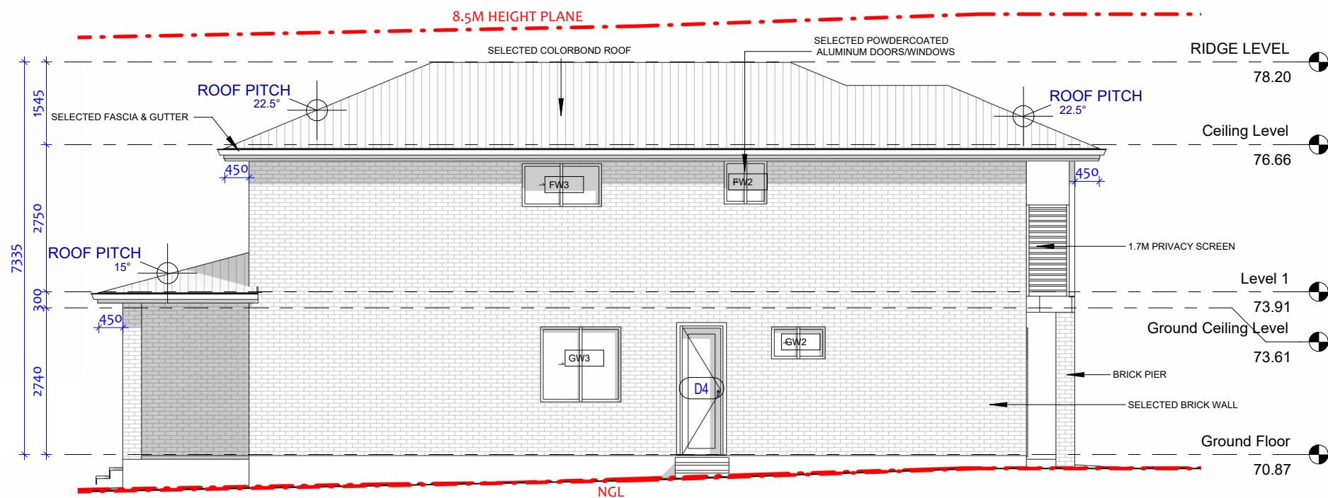
2 West Elevation 1 : 100
