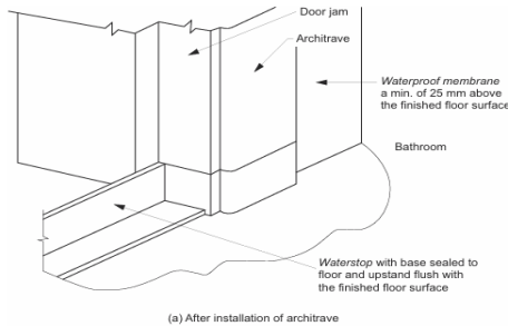
(a) After installation of architrave
