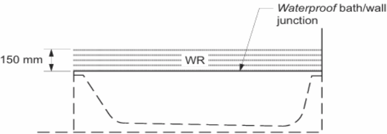
(b) Wall/bath junction
