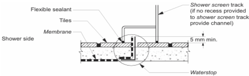
Figure 10.2.17: Typical hobless construction
