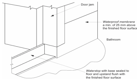
(b) Prior to installation of architrave
