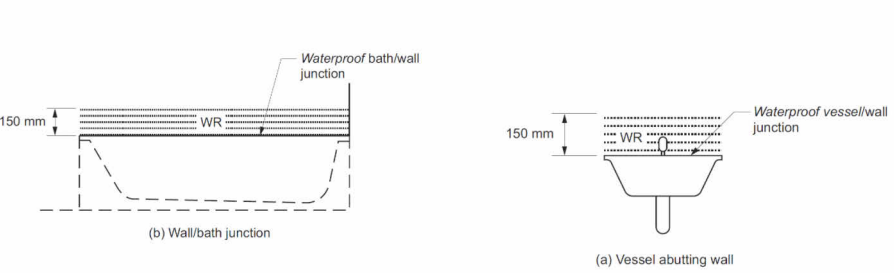
Figure 10.2.5: Bath and vessel abutting wall - areas to be protected
