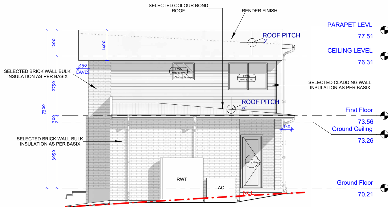
SOUTH ELEVATION
