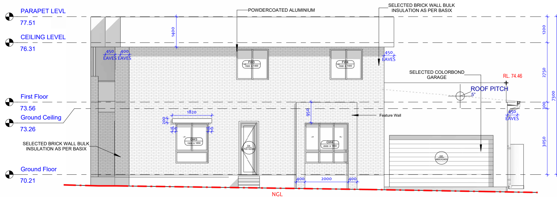
WEST ELEVATION
