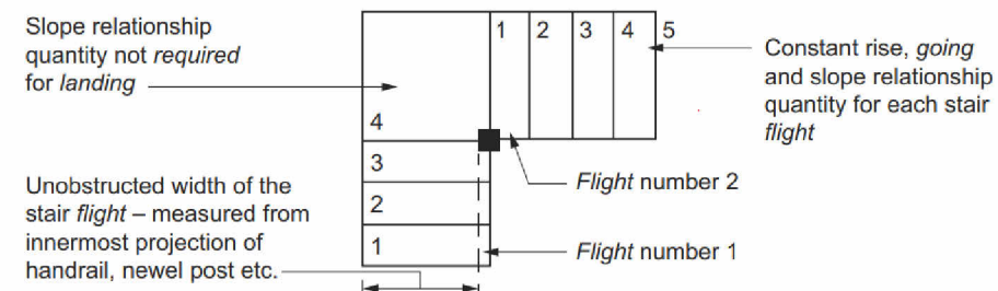
Figure 11.2.2a: Measurement of slope relationship — Plan view — Stair with 2 flights
