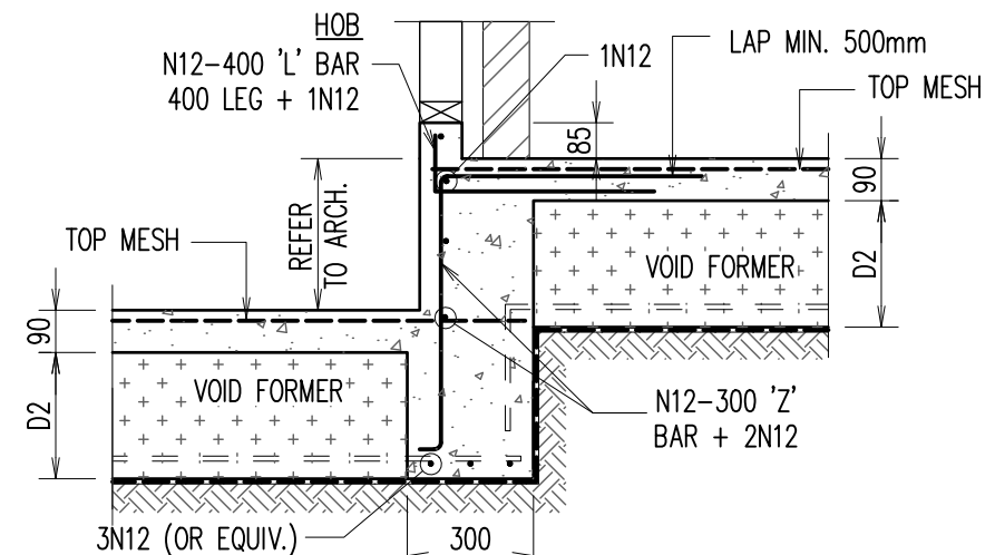
INTERNAL STEPDOWN BEAM - 'IB4'
