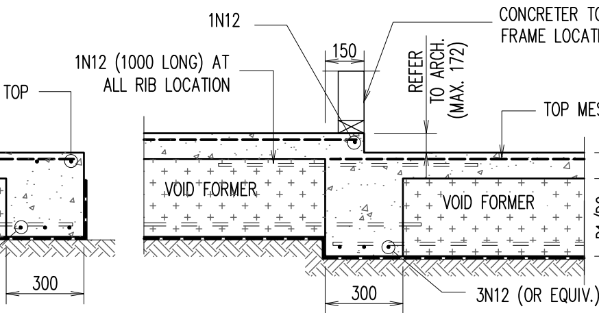
INTERNAL STEPDOWN BEAM - 'IB3'
